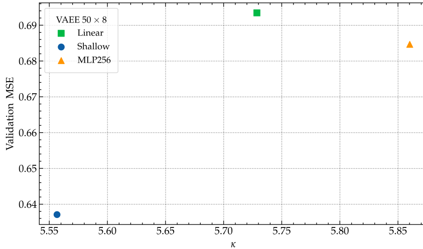
Figure 4.5: Validation MSE of the VAE under encoder and decoder architectures of increasing depth — a plain linear encoder, the shallow linear-plus-GELU encoder used throughout, and an MLP with a hidden layer 256 neurons wide — at a fixed dictionary size K = 50 and embedding width d = 8 . The shallow configuration achieves better reconstruction at a lower \kappa than both the linear and MLP configurations.
