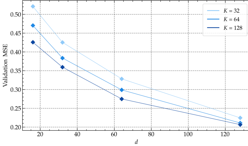
Figure 4.5: Effect of the per-concept embedding width d on VAAE reconstruction. Validation MSE against d \in \{16, 32, 64, 128\} , one curve per dictionary size K \in \{32, 64, 128\} , all at the fixed sparsity target \tilde{\kappa} = \pi K = 8 , so that only the embedding width varies along each curve. Reconstruction improves with d , with diminishing returns — widening a concept adds capacity that a scalar atom cannot, though at the cost of more active neurons ( \ell_0 = \kappa d ) and more parameters.
