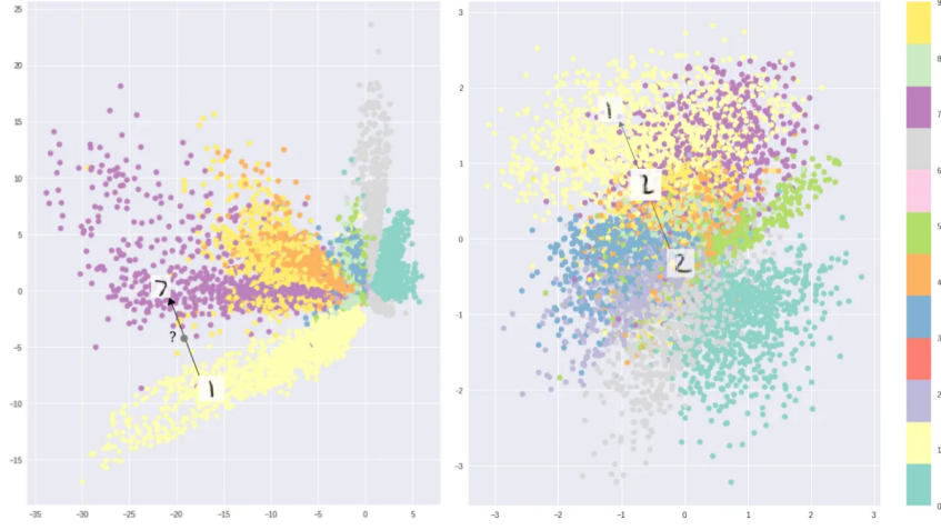
Figure 2.2: Two-dimensional latent spaces learned on MNIST, coloured by digit class, reproduced from Shafkat [33]. Optimising for reconstruction alone (left) lets a standard autoencoder separate the classes into disconnected clusters with gaps that decode to unrealistic samples, whereas the Variational AutoEncoder objective (right) yields a smoother, more continuous arrangement, concentrated around the origin by the prior, that can be sampled and interpolated.
