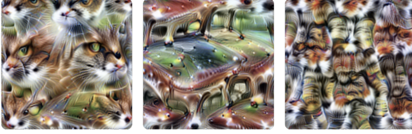
Figure 2.3: Neuron 4e:55, a polysemantic neuron from InceptionV1 which responds to cat faces, fronts of cars, and cat legs. Reproduced from Olah et al. [23].
