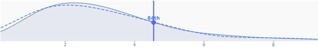
DISTRIBUTION · Czech I (blue dashed) vs Czech I+II (grey)
