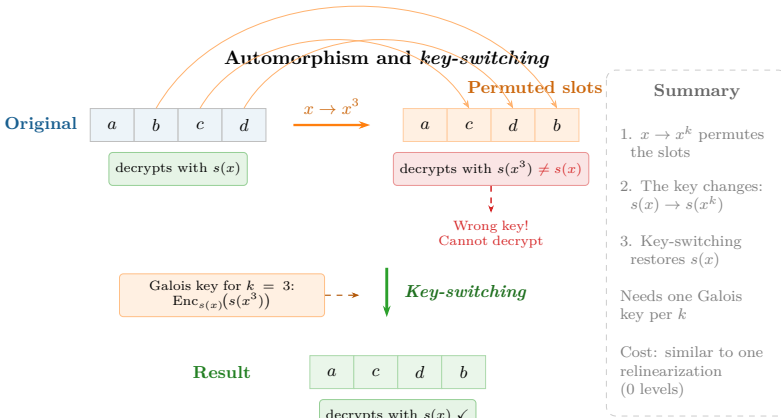
Figure 5.13: Automorphism and key-switching. The substitution x \rightarrow x^k permutes the ciphertext’s slots, but changes the decryption key from s(x) to s(x^k) . Key-switching, using a precomputed Galois key, restores the original key without revealing the secret.
