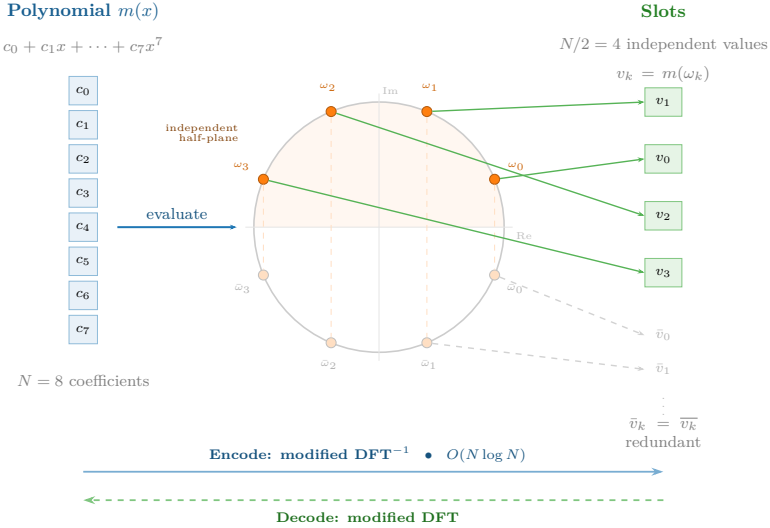
Figure 5.10: Canonical embedding. The polynomial m(x) ’s coefficients are not the data: the slots are the evaluations of m(x) at the N complex roots of x^N + 1 . Conjugate roots produce redundant values, leaving N/2 independent slots. Encoding and decoding are equivalent to a modified DFT (inverse and direct, respectively).
