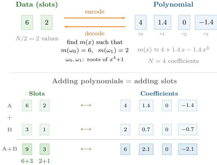
Figure 5.11: Slot-based encoding ( N = 4 ). Above: two data points [6, 2] are encoded as a polynomial with 4 coefficients by finding m(x) such that m(\omega_0) = 6 and m(\omega_1) = 2 . Below: adding two polynomials coefficient by coefficient is equivalent to adding the slots element by element — the basis of SIMD parallelism.
