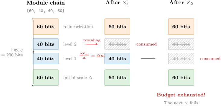
Figure 5.7: Modulus chain and level consumption. Left: the initial chain [60, 40, 40, 60] with its four links — the top 60-bit link reserved for relinearization, the two 40-bit links serving as available multiplication levels, and the bottom 60-bit link fixing the initial scale \Delta . Center: after the first multiplication, rescaling divides by \Delta and consumes the “level 2” link, leaving one available. Right: after the second multiplication, “level 1” is also consumed and the budget is exhausted — a third multiplication would have no link left to consume and would fail.
