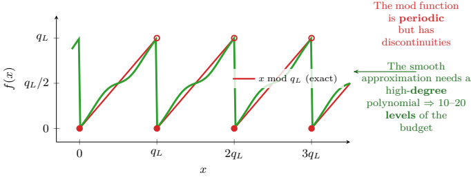
Figure 5.8: Approximation of modular reduction. The function “ x modulo q_L ” is periodic but discontinuous — it cannot be expressed as a sequence of additions and multiplications. To evaluate it homomorphically, it is approximated by a high-degree polynomial, which consumes between 10 and 20 multiplicative levels.
