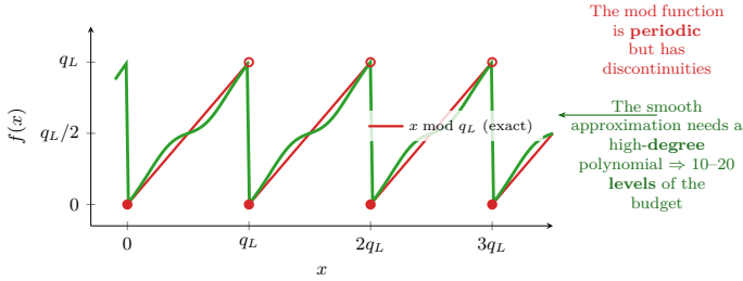
Figure 5.8: Approximation of modular reduction. The function “ x modulo q_L ” is periodic but discontinuous — it cannot be expressed as a sequence of additions and multiplications. To evaluate it homomorphically, it is approximated by a high-degree polynomial, which consumes between 10 and 20 multiplicative levels.
