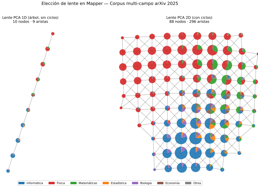
Figure 1.10: Comparison of Mapper lenses on the arXiv 2025 corpus (8,085 articles). Left: 1D PCA lens — tree with 10 nodes and 9 edges, no cycles. Right: 2D PCA lens — network with 88 nodes and 296 edges with interdisciplinary cycles. Same color palette as in Figure 1.11.
