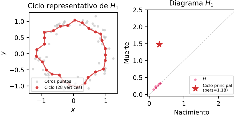
Figure 1.7: Recipe 4: representative cycle of the main hole. Left: the cycle's vertices (red) and their edges form a closed polygon enclosing the empty central region of the ring; the other points appear in gray. Right: H_1 persistence diagram with the star marking the extracted feature.
