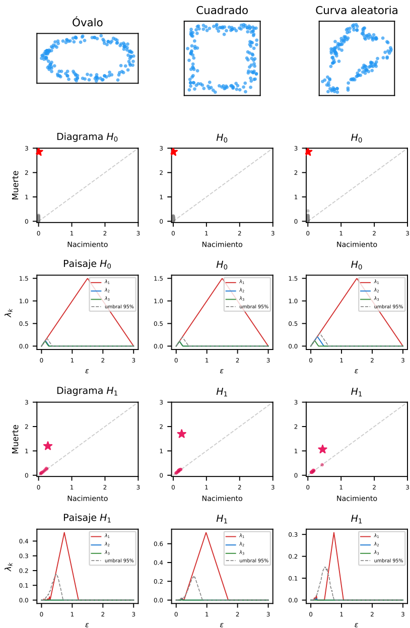
Figure 1.4: Topological invariance: an oval, a square, and a random curve — three different geometries with the same topology. In all cases, H_0 detects one component and H_1 detects a persistent cycle (star). The geometric shape changes; the topological shape does not.
