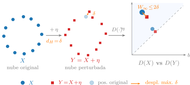
Figure 1.20: Illustration of the stability theorem in three steps. Left: original point cloud X (blue points). Center: perturbed point cloud Y = X + \eta ; the faded point shows the original position; the orange arrow marks the worst displacement \delta = d_H(X, Y) . Right: persistence diagrams D(X) (circles) and D(Y) (squares) overlaid; the gray lines show the optimal bottleneck matching; the orange arrow bounds the largest displacement in PD space, which cannot exceed W_\infty \leq 2\delta .
