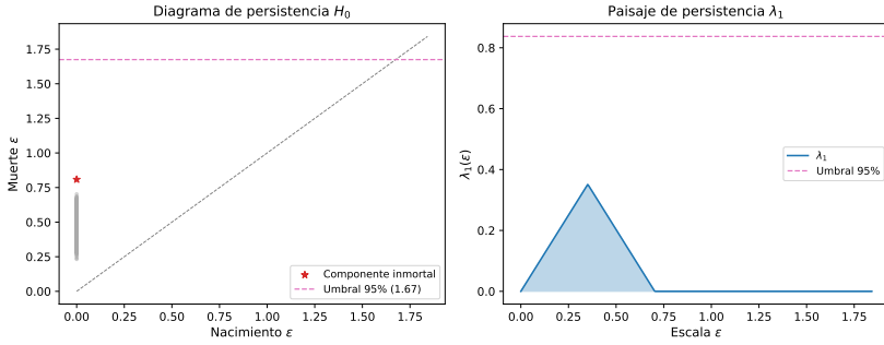
Figure 1.9: H_0 analysis of the multi-field corpus (8,085 arXiv 2025 articles, 29 categories). Left: persistence diagram — all points near the diagonal, no bar exceeds the 95% threshold. Right: \lambda_1 landscape with null threshold (dashed line). ArXiv science is a single connected component at the level of statistical significance.
