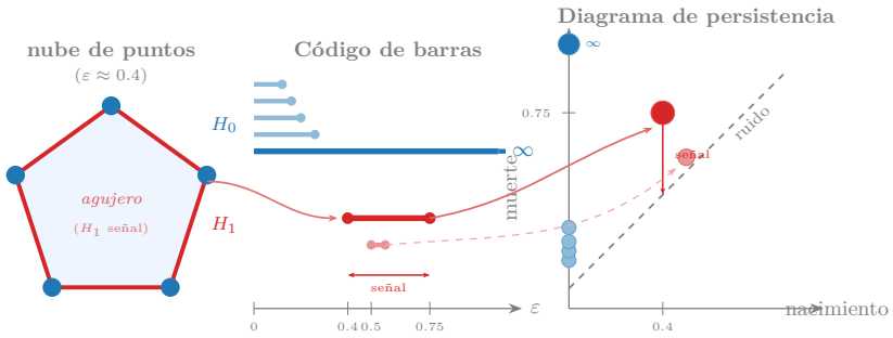
Figure 1.19: Left: five points arranged in a regular pentagon at scale \varepsilon \approx 0.4 — the edges (red) form a closed loop and the shaded interior is the hole that gives rise to the H_1 feature. Center: barcode of the point cloud; the four short blue bars are H_0 noise (components that merge quickly), the long blue bar with an arrow is the immortal H_0 , the long red bar is the H_1 signal (the hole), and the very short red bar is H_1 noise. Right: persistence diagram; the small blue points near the diagonal are H_0 noise, the large red point far from the diagonal is the H_1 signal, and the small red point next to the diagonal is H_1 noise. Distance to the diagonal axis measures persistence: signal above, noise below. Arrows show the bar — point correspondence.
