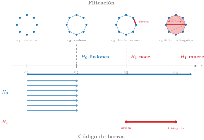
Figure 1.18: Four frames of the filtration synchronized with the barcode. \varepsilon_2 : edges form a chain ( \beta_0 = 1 , \beta_1 = 0 ). \varepsilon_3 : the red edge closes the loop — H_1 is born ( \beta_1 = 1 ). \varepsilon_4 : when \varepsilon reaches the diameter ( 2r ), the fan-shaped triangles — formed using only ring points, with no central point — fill the interior and H_1 dies ( \beta_1 = 0 ). The diameter (thick red line) is the critical chord.
