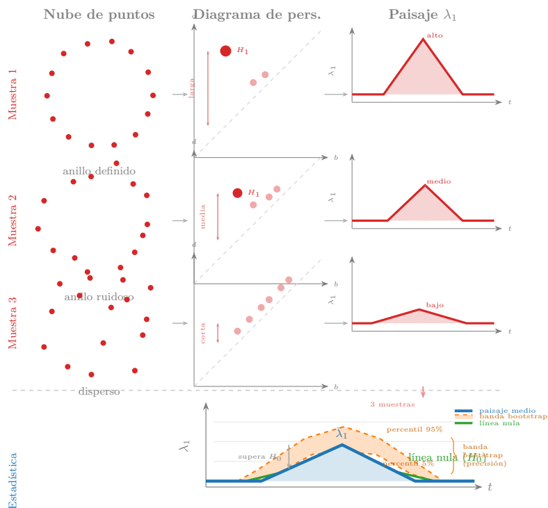
Figure 1.22: Three samples from the same process (rows 1–3) produce persistence diagrams with bars of different lengths and landscapes with peaks of different heights. The bottom row overlays the three individual landscapes (red) to obtain the mean landscape (blue), the bootstrap band 5%–95% (orange, variability band from resamples of the original dataset), and the null line (green, 95th percentile of landscapes from permuted data). The blue peak exceeds the null line — statistically significant signal — and stays within the bootstrap band — reproducible signal.
