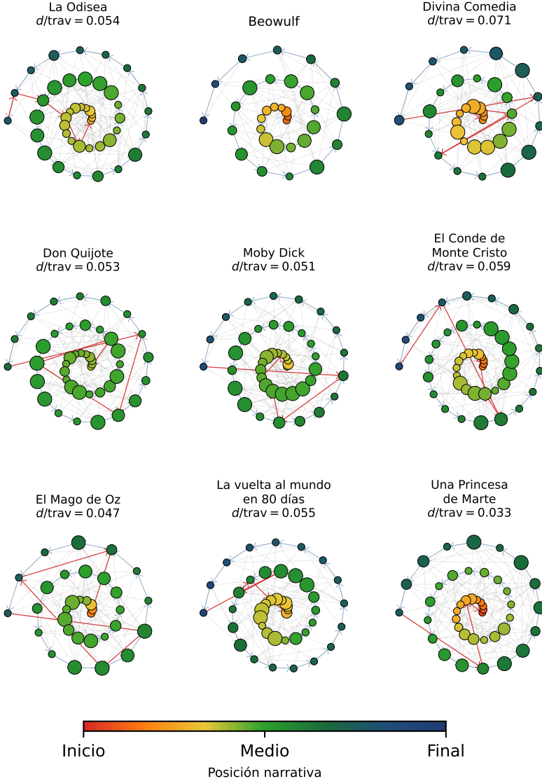
Figure 1.8: Recipe 5: spiral hypergraph of nine classic novels. Each node is a semantic cluster; its area is proportional to the fraction of passages it contains, and its position on the spiral reflects narrative order (center = beginning, outer = end). Blue arrows: chronological traversal. Red arrows: return path via semantic edges. The ratio d/\text{trav} measures the relative cost of the return.
