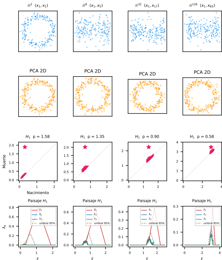
Figure 1.6: Curse of dimensionality: circle of R = 1.5 embedded in \mathbb{R}^2 , \mathbb{R}^8 , \mathbb{R}^{32} , and \mathbb{R}^{128} with noise \sigma = 0.2 . Row 1: projection (x_1, x_{d/2+1}) — in high dimension, a coordinate of pure noise. Row 2: PCA 2D — recovers the circle in all cases (ideal scenario for PCA). Row 3: H_1 diagram — the most persistent star approaches the diagonal. Row 4: \lambda_1 landscape — the signal-to-noise ratio decreases; in \mathbb{R}^{128} the H_1 peaks are barely distinguishable from the permutation threshold.
