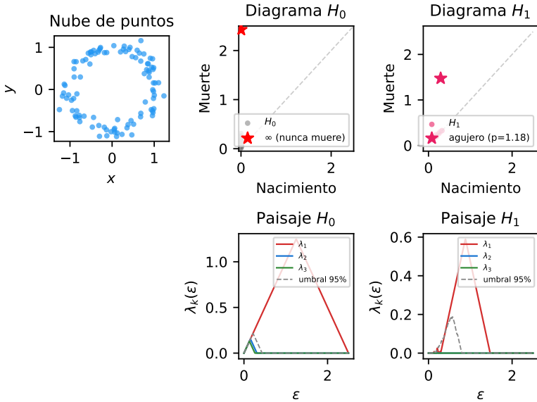
Figure 1.3: Recipe 2: above, point cloud on a circle with noise, H_0 persistence diagram and H_1 diagram — the pink star is the central hole, far from the diagonal. Below, landscapes with the 95% threshold (dashed line): in H_0 , \lambda_1 stands out (the immortal component) but \lambda_2 and \lambda_3 don't — there's a single piece; in H_1 , \lambda_1 clearly surpasses the threshold, confirming that the hole is signal.
