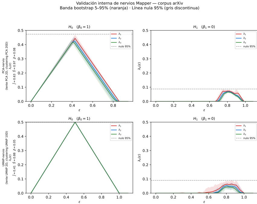
Figure 1.15: Internal validation of the two Mapper nerves on the arXiv corpus. Each panel shows the mean persistence landscape (lines) with the 5–95% bootstrap band (shading) and the 95% null line (dashed gray) for H_0 and H_1 . H_2 is not computed: with a 2D lens it is structurally zero (see Section 1.6.8). The legend in each row includes \bar{J} , \bar{S} , and \rho (mean density of the bootstrap nerve, parameter of the null binomial model used to compute the z-score of \bar{S} ).
