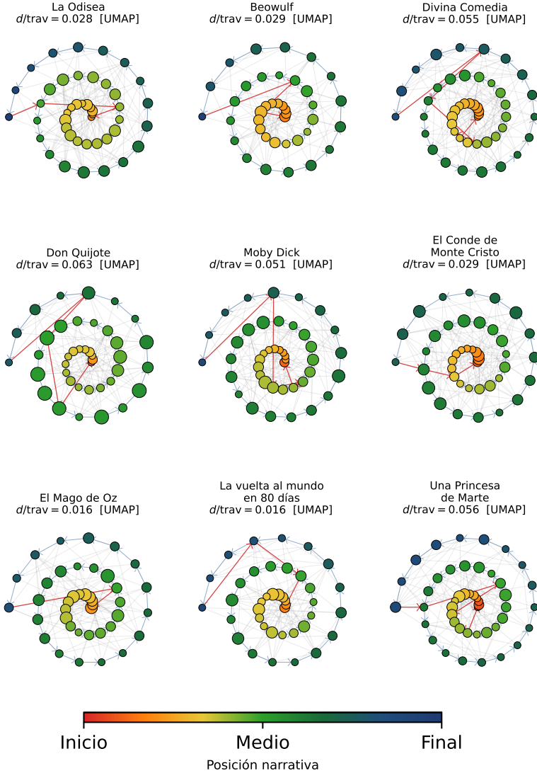
Figure 1.13: Recipe 8 (hero's journey): spiral hypergraph with 2D UMAP lens and 10D UMAP clustering, both reductions independent. The non-linear lens groups within each patch passages that PCA would separate; nodes are placed on the spiral according to their mean narrative position (center = beginning, outer edge = end). The red arrows (return) still cross nearly the entire graph, confirming that the beginning and end are semantically distant in all nine novels.
