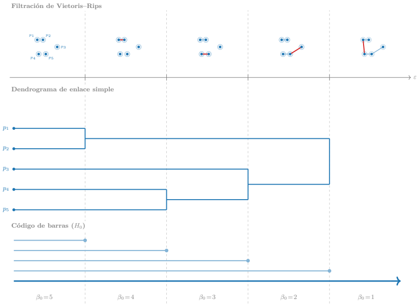
Figure 1.17: Vietoris-Rips filtration over five points (top), single-linkage dendrogram (middle), and H_0 barcode (bottom), aligned on the same scale \varepsilon . Each frame shows the edge that triggers the merge (in red); the number \beta_0 indicates how many connected components remain active between events. The immortal bar (arrow) is the component that persists forever.
