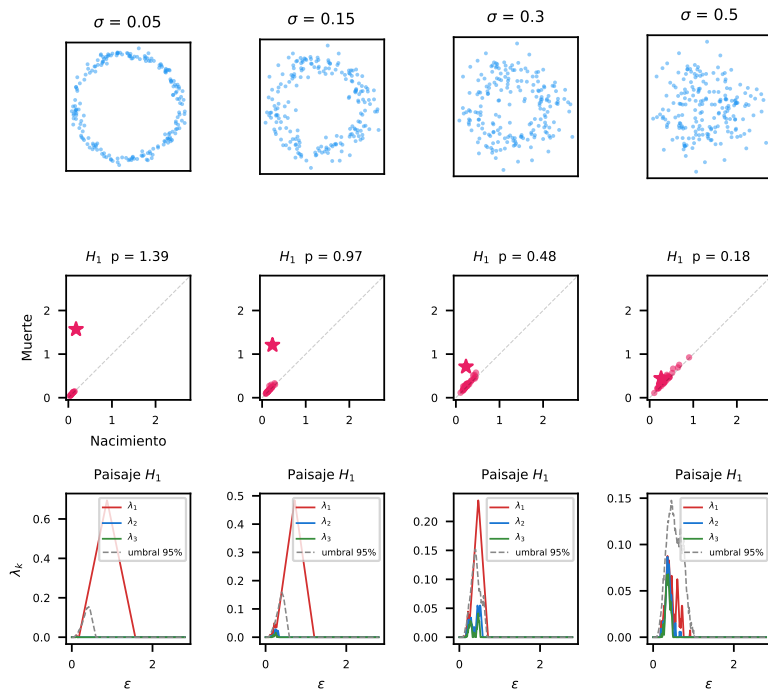
Figure 1.5: Recipe 3 — stability: above, the same circle with four increasing noise levels ( \sigma ); middle, H_1 persistence diagram (the star marks the main hole); below, persistence landscape \lambda_1 with the 95% threshold. The signal decreases gradually — it never disappears abruptly.
