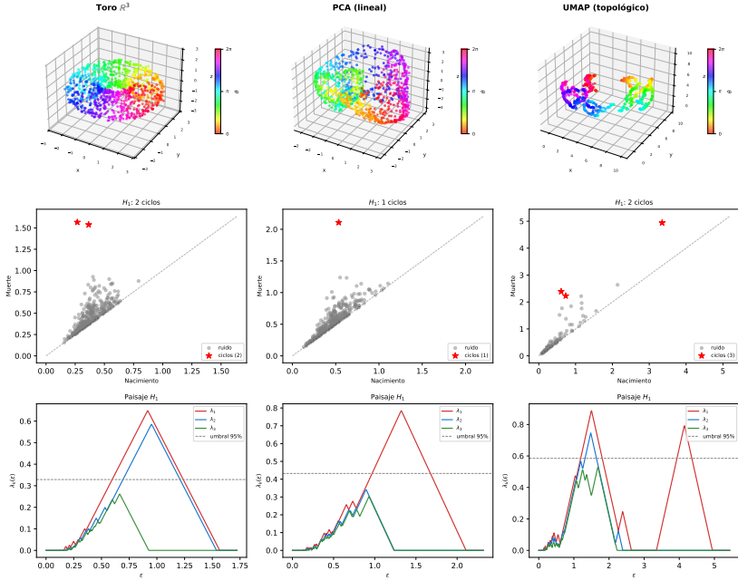
Figure 1.12: Recipe 7: reduction of a torus ( \beta_1 = 2 ) from \mathbb{R}^{50} to \mathbb{R}^3 with PCA (center column) and UMAP (right column), with the original torus in \mathbb{R}^3 as reference (left column). Top row: 3D point clouds colored by \theta — PCA may look geometrically clean, UMAP often looks distorted: both appearances are misleading. Middle row: H_1 persistence diagram, red stars = persistent cycles; PCA detects 1, UMAP detects 2. Bottom row: persistence landscape with layers \lambda_1 (red) and \lambda_2 (blue), 95% null threshold (dashed line) — only UMAP has both layers above the threshold, confirming \beta_1 = 2 .
