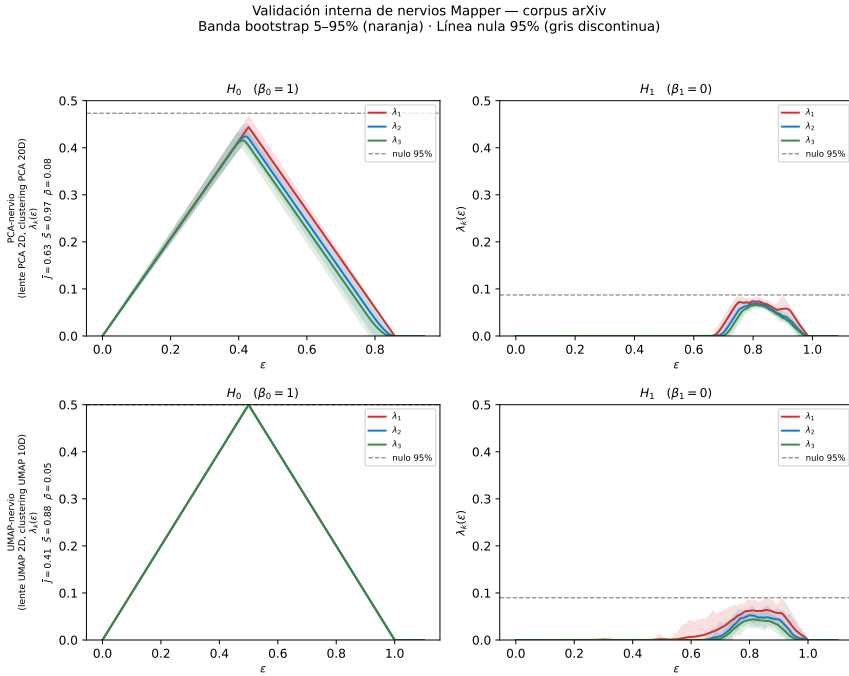
Figure 2.15: Internal validation of the two Mapper nerves on the arXiv corpus. Each panel shows the mean persistence landscape (lines) with the 5–95% bootstrap band (shading) and the 95% null line (dashed gray) for H_0 and H_1 . H_2 is not computed: with a 2D lens it is structurally zero (see Section 5.8). The legend in each row includes \bar{J} , \bar{S} , and \rho (mean density of the bootstrap nerve, parameter of the null binomial model used to compute the z-score of \bar{S} ).
