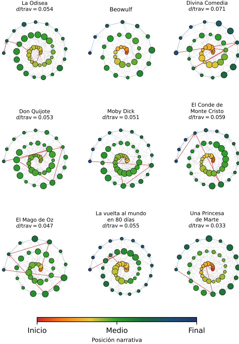
Figure 2.8: Recipe 5: spiral hypergraph of nine classic novels. Each node is a semantic cluster; its area is proportional to the fraction of passages it contains, and its position on the spiral reflects narrative order (center = beginning, outer = end). Blue arrows: chronological traversal. Red arrows: return path via semantic edges. The ratio d/trav measures the relative cost of the return.
