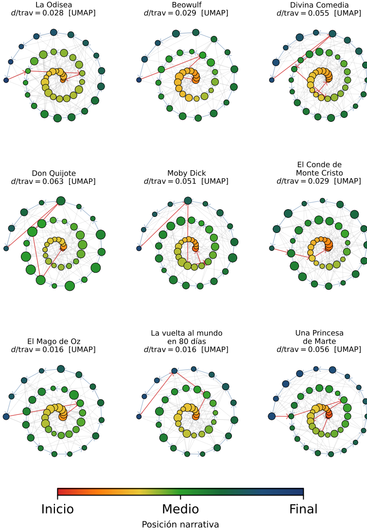
Figure 2.13: Recipe 8 (hero's journey): spiral hypergraph with 2D UMAP lens and 10D UMAP clustering, both reductions independent. The non-linear lens groups within each patch passages that PCA would separate; nodes are placed on the spiral according to their mean narrative position (center = beginning, outer edge = end). The red arrows (return) still cross nearly the entire graph, confirming that the beginning and end are semantically distant in all nine novels.
