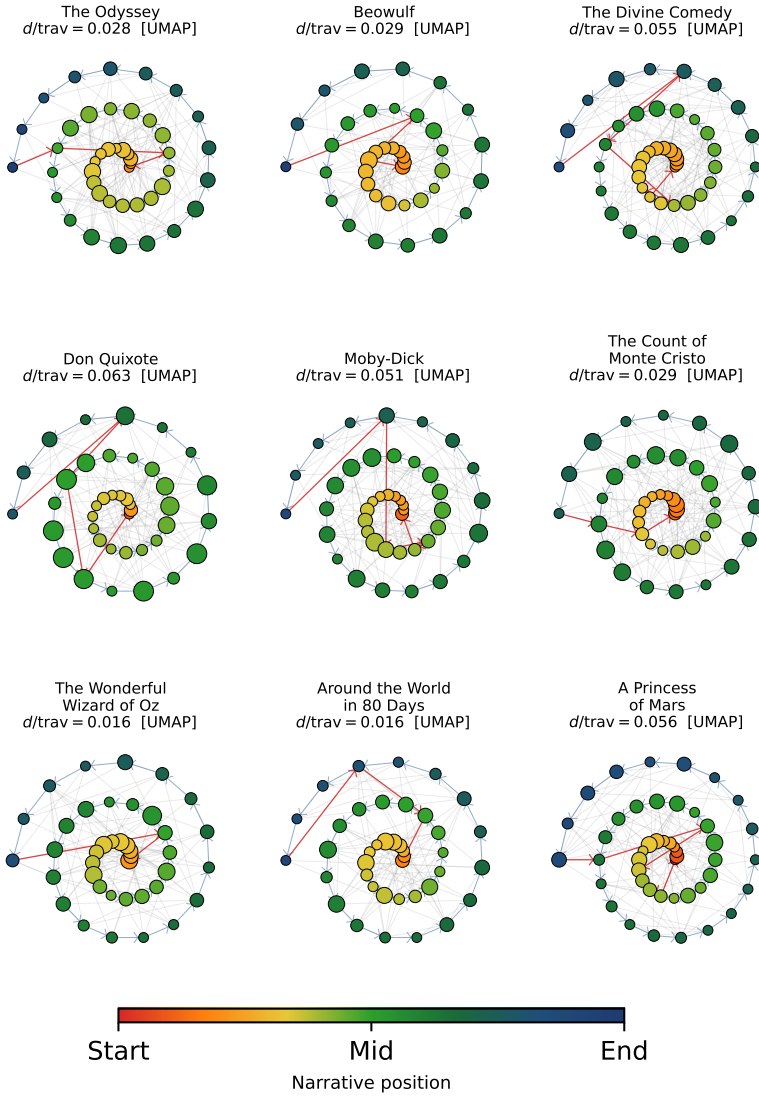
Figure 2.13: Recipe 8 (hero's journey): spiral hypergraph with 2D UMAP lens and DBSCAN with cosine distance on the original embeddings in \mathbb{R}^{384} . The non-linear lens organizes Mapper's patches; nodes are placed on the spiral according to their mean narrative position (center = beginning, outer edge = end). The red arrows (return) still cross nearly the entire graph, confirming that the beginning and end are semantically distant in all nine novels.
