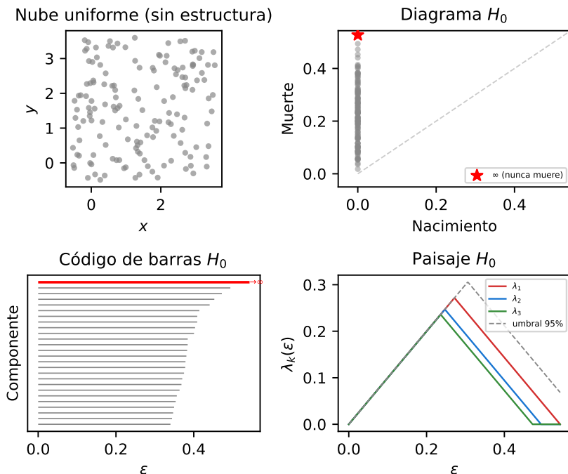
Figure 2.2: Negative control: 150 uniform points (no structure). The diagram, barcode, and persistence landscape show only noise — \lambda_1 barely surpasses the null threshold, without the prominent peaks from Figure 2.1.
