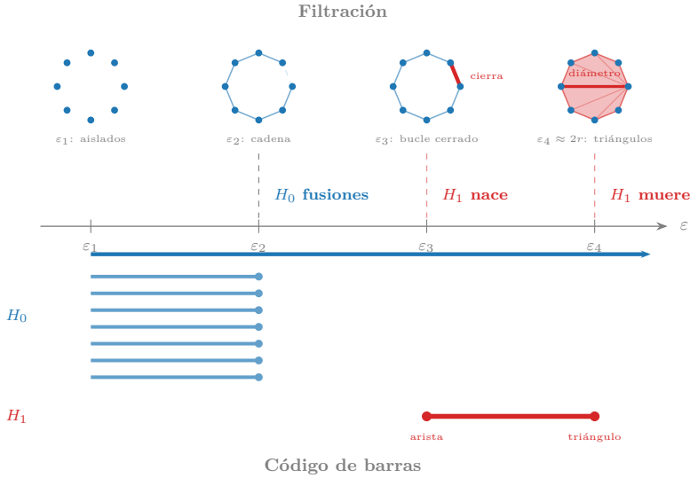
Figure 5.3: Four frames of the filtration synchronized with the barcode. \varepsilon_2 : edges form a chain ( \beta_0 = 1 , \beta_1 = 0 ). \varepsilon_3 : the red edge closes the loop — H_1 is born ( \beta_1 = 1 ). \varepsilon_4 : when \varepsilon reaches the diameter ( 2r ), the fan-shaped triangles — formed using only ring points, with no central point — fill the interior and H_1 dies ( \beta_1 = 0 ). The diameter (thick red line) is the critical chord.
