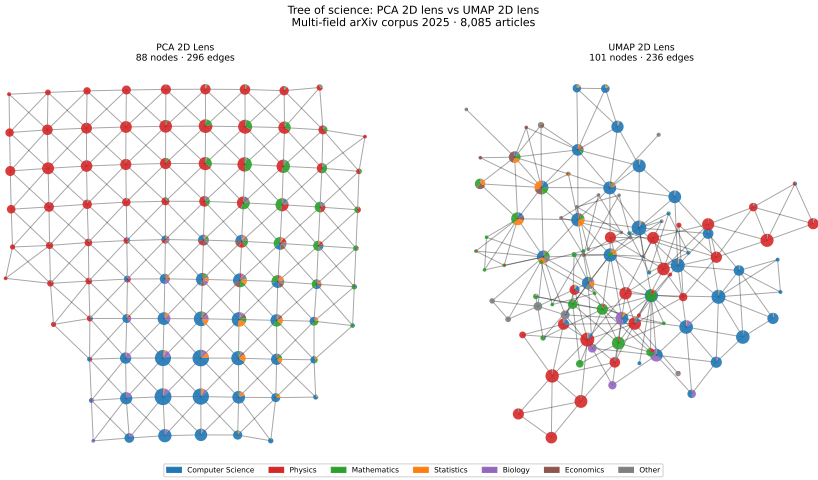
Figure 2.14: Recipe 8 (tree of science): comparison of Mapper lenses on the arXiv 2025 corpus. Left: 2D PCA lens with 20D PCA clustering — 88 nodes and 296 edges. Right: 2D UMAP lens with cosine DBSCAN on \mathbb{R}^{384} — 101 nodes and 236 edges. With UMAP, disciplines cluster geographically according to the non-linear manifold of the corpus: fields with more similar vocabulary appear adjacent, and multicolored nodes (interdisciplinary bridges) concentrate in the transition zones.
