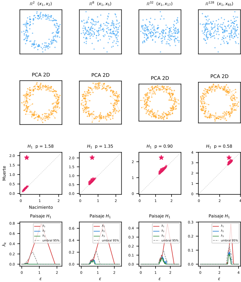
Figure 2.6: Curse of dimensionality: circle of R = 1.5 embedded in \mathbb{R}^2 , \mathbb{R}^8 , \mathbb{R}^{32} , and \mathbb{R}^{128} with noise \sigma = 0.2 . Row 1: projection (x_1, x_{d/2+1}) — in high dimension, a coordinate of pure noise. Row 2: PCA 2D — recovers the circle in all cases (ideal scenario for PCA). Row 3: H_1 diagram — the most persistent star approaches the diagonal. Row 4: \lambda_1 landscape — the signal-to-noise ratio decreases; in \mathbb{R}^{128} the H_1 peaks are barely distinguishable from the permutation threshold.
