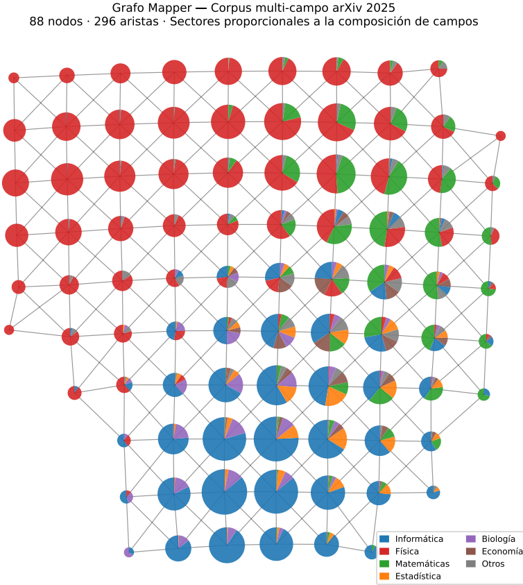
Figure 2.11: Mapper graph of the multi-field arXiv 2025 corpus (8,085 articles, 88 nodes, 2D PCA lens). Each node is drawn as a pie chart with sectors proportional to the field composition (blue = Computer Science, red = Physics, green = Mathematics, orange = Statistics, purple = Biology, brown = Economics). Size is proportional to the number of papers. Single-color nodes are monodisciplinary; multi-color nodes are interdisciplinary bridges.
