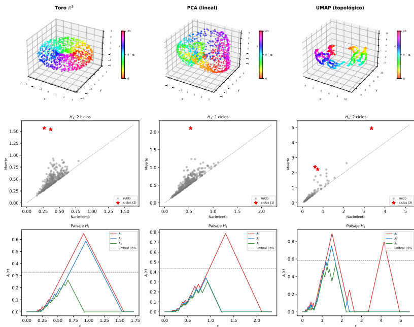
Figure 2.12: Recipe 7: reduction of a torus ( \beta_1 = 2 ) from \mathbb{R}^{50} to \mathbb{R}^3 with PCA (center column) and UMAP (right column), with the original torus in \mathbb{R}^3 as reference (left column). Top row: 3D point clouds colored by \theta — PCA may look geometrically clean, UMAP often looks distorted: both appearances are misleading. Middle row: H_1 persistence diagram, red stars = persistent cycles; PCA detects 1, UMAP detects 2. Bottom row: persistence landscape with layers \lambda_1 (red) and \lambda_2 (blue), 95% null threshold (dashed line) — only UMAP has both layers above the threshold, confirming \beta_1 = 2 .
