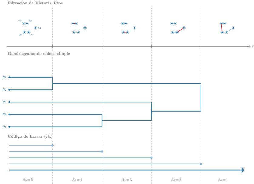
Figure 5.2: Vietoris-Rips filtration over five points (top), single-linkage dendrogram (middle), and H_0 barcode (bottom), aligned on the same scale \varepsilon . Each frame shows the edge that triggers the merge (in red); the number \beta_0 indicates how many connected components remain active between events. The immortal bar (arrow) is the component that persists forever.
