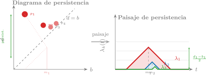
Figure 5.6: From persistence diagram to landscape. Each point (b_i, d_i) in the PD generates a tent function \Lambda_i (left panel, colored by persistence). The landscape \lambda_k takes the k -th maximum at each scale t (right panel). Levels \lambda_1, \lambda_2, \lambda_3 capture signal of decreasing persistence: \lambda_1 reflects the dominant feature, \lambda_2 the secondary one.
