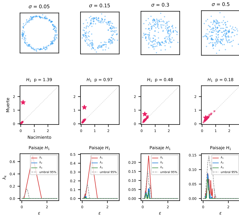
Figure 2.5: Recipe 3 — stability: above, the same circle with four increasing noise levels ( \sigma ); middle, H_1 persistence diagram (the star marks the main hole); below, persistence landscape \lambda_1 with the 95% threshold. The signal decreases gradually — it never disappears abruptly.
