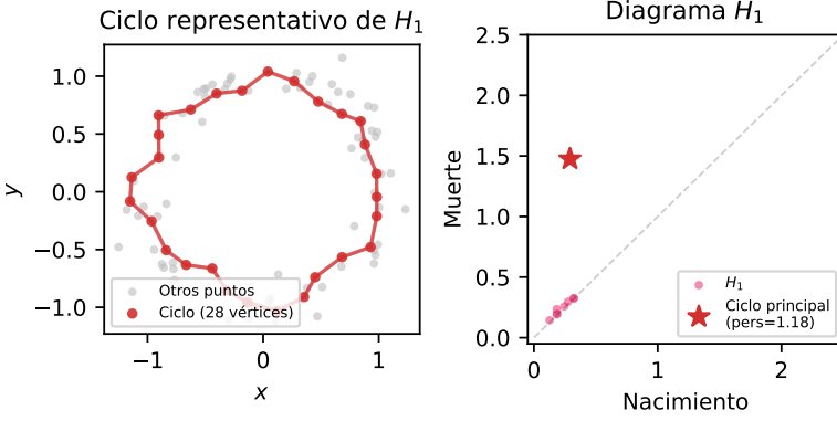
Figure 2.7: Recipe 4: representative cycle of the main hole. Left: the cycle’s vertices (red) and their edges form a closed polygon enclosing the empty central region of the ring; the other points appear in gray. Right: H_1 persistence diagram with the star marking the extracted feature.
