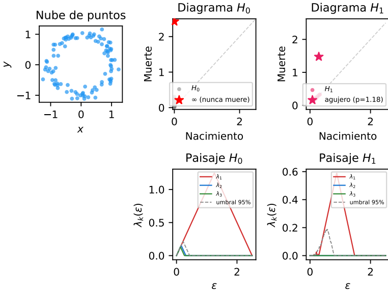
Figure 2.3: Recipe 2: above, point cloud on a circle with noise, H_0 persistence diagram and H_1 diagram — the pink star is the central hole, far from the diagonal. Below, landscapes with the 95% threshold (dashed line): in H_0 , \lambda_1 stands out (the immortal component) but \lambda_2 and \lambda_3 don't — there's a single piece; in H_1 , \lambda_1 clearly surpasses the threshold, confirming that the hole is signal.
