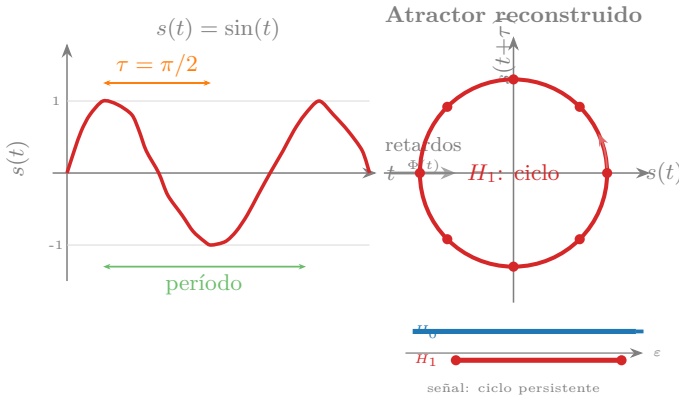
Figure 5.9: Delay embedding of s(t) = \sin(t) with delay \tau = \pi/2 . Left: the scalar signal s(t) vs. t . Right: the trajectory (s(t), s(t+\tau)) in \mathbb{R}^2 traces a clean circle. The mini-barcode below shows an immortal component in H_0 and a highly persistent cycle in H_1 — the topological signature of periodicity.
