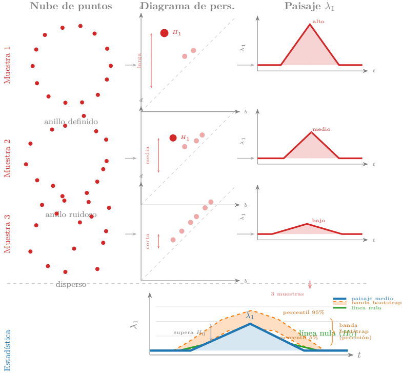
Figure 5.7: Three samples from the same process (rows 1–3) produce persistence diagrams with bars of different lengths and landscapes with peaks of different heights. The bottom row overlays the three individual landscapes (red) to obtain the mean landscape (blue), the bootstrap band 5%–95% (orange, variability band from resamples of the original dataset), and the null line (green, 95th percentile of landscapes from permuted data). The blue peak exceeds the null line — statistically significant signal — and stays within the bootstrap band — reproducible signal.
