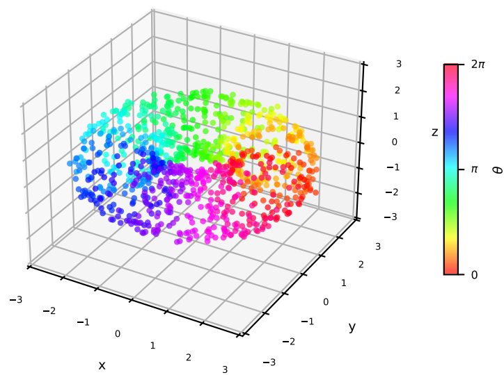
Toro \mathbb{R}^3
