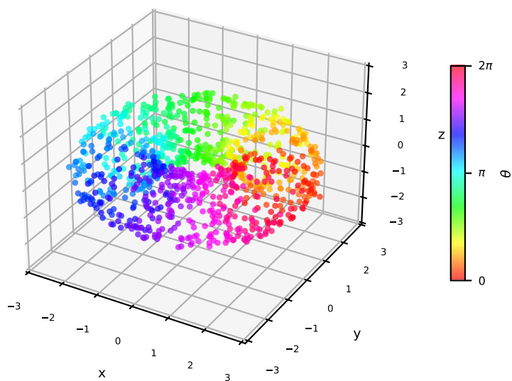
Toro \mathbb{R}^3
