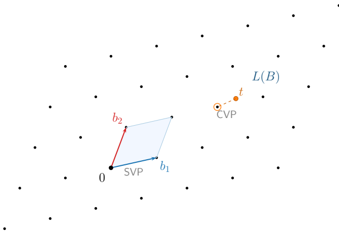
Figure 3.1: Two-dimensional lattice generated by two basis vectors b_1 and b_2 . The shaded region is the fundamental domain (parallelogram defined by the basis). The point t lies outside the lattice: finding the nearest lattice point (CVP) or the shortest nonzero vector (SVP) is computationally intractable in high dimensions.
