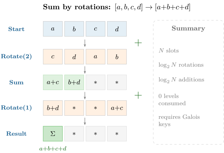
Figure 3.12: Summation via rotations. With 4 slots, two rotate-and-add steps suffice to accumulate the total sum in the first slot. The diagram shows the slot-level view; internally, each “Add” is an addition of the N coefficients of two polynomials, which by linearity of evaluation produces the slot-by-slot sum. Rotations require Galois keys but do not consume multiplicative levels.
