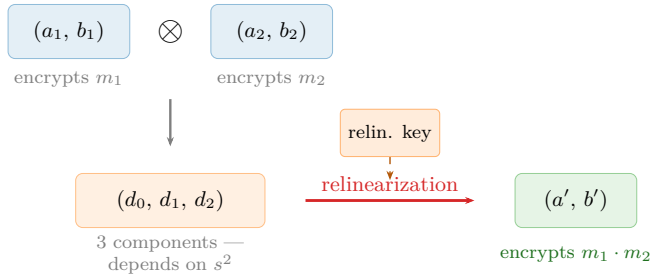
Figure 3.5: Multiplication between ciphertexts. The product generates a triplet (d_0, d_1, d_2) that depends on s^2 . Relinearization, using a public key that encrypts s^2 , reduces it to a standard pair (a', b') decryptable with s .
