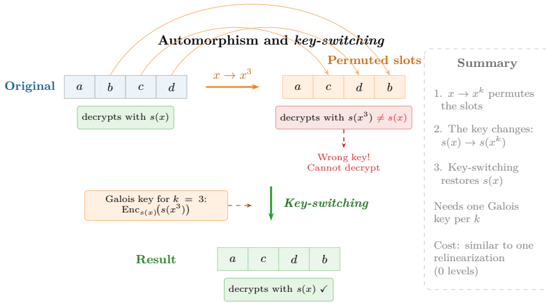
Figure 3.13: Automorphism and key-switching. The substitution x \rightarrow x^k permutes the ciphertext’s slots, but changes the decryption key from s(x) to s(x^k) . Key-switching, using a precomputed Galois key, restores the original key without revealing the secret.
