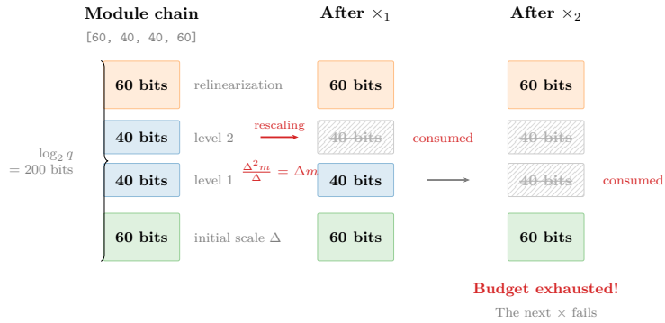
Figure 3.7: Modulus chain and level consumption. Each multiplication consumes one 40-bit link via rescaling. When the intermediate links run out, the next multiplication fails.
