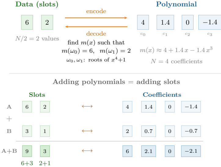
Figure 3.11: Slot-based encoding ( N = 4 ). Above: two data points [6, 2] are encoded as a polynomial with 4 coefficients by finding m(x) such that m(\omega_0) = 6 and m(\omega_1) = 2 . Below: adding two polynomials coefficient by coefficient is equivalent to adding the slots element by element — the basis of SIMD parallelism.
