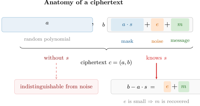
Figure 3.4: Anatomy of a ciphertext. The pair (a, b) contains the message m hidden behind a mask a \cdot s and noise e . Anyone who knows s removes the mask and recovers m ; without s , the ciphertext is indistinguishable from random noise.
