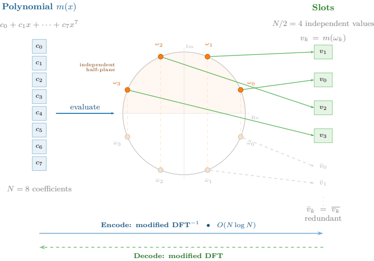
Figure 3.10: Canonical embedding. The polynomial m(x) ’s coefficients are not the data: the slots are the evaluations of m(x) at the N complex roots of x^N + 1 . Conjugate roots produce redundant values, leaving N/2 independent slots. Encoding and decoding are equivalent to a modified DFT (inverse and direct, respectively).
