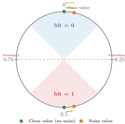
Figure 3.14: Encoding on the torus \mathbb{T} = \mathbb{R}/\mathbb{Z} . Bit 0 is encoded near 0.0 (top) and bit 1 near 0.5 (bottom). Noise displaces the position, but the bit is recovered as long as it doesn’t cross the decision boundary (0.25 or 0.75).
