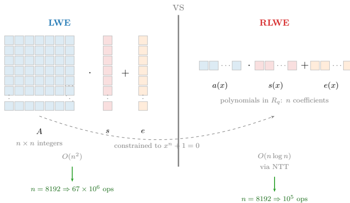
Figure 3.3: LWE versus RLWE. On the left, LWE requires an n \times n integer matrix A . On the right, RLWE encodes the same information in a polynomial of n coefficients, reducing the cost from O(n^2) to O(n \log n) via the NTT.
