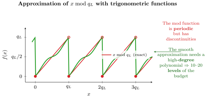
Figure 3.8: Approximation of modular reduction. The function “ x modulo q_L ” is periodic but discontinuous — it cannot be expressed as a sequence of additions and multiplications. To evaluate it homomorphically, it is approximated by a high-degree polynomial, which consumes between 10 and 20 multiplicative levels.
