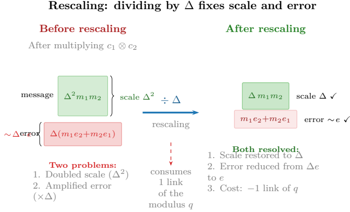
Figure 3.6: Rescaling: dividing by \Delta simultaneously corrects the doubled scale and the amplified error, at the cost of consuming one link of the modulus chain.
