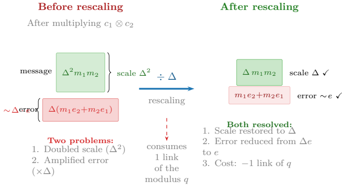
Figure 4.6: Rescaling: dividing by \Delta simultaneously corrects the doubled scale and the amplified error, at the cost of consuming one link of the modulus chain.
