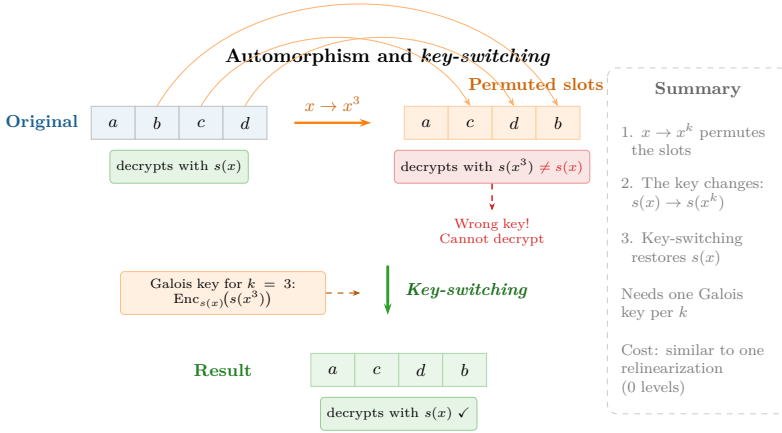
Figure 4.13: Automorphism and key-switching. The substitution x \rightarrow x^k permutes the ciphertext’s slots, but changes the decryption key from s(x) to s(x^k) . Key-switching, using a precomputed Galois key, restores the original key without revealing the secret.
