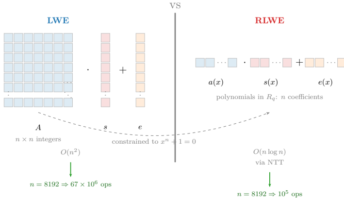
Figure 4.3: LWE versus RLWE. On the left, LWE requires an n \times n integer matrix A . On the right, RLWE encodes the same information in a polynomial of n coefficients, reducing the cost from O(n^2) to O(n \log n) via the NTT.
