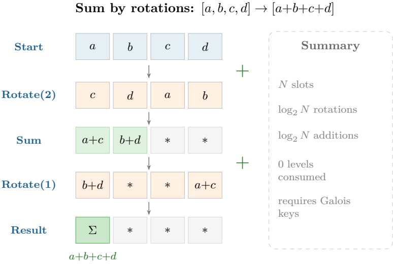
Figure 4.12: Summation via rotations. With 4 slots, two rotate-and-add steps suffice to accumulate the total sum in the first slot. The diagram shows the slot-level view; internally, each “Add” is an addition of the N coefficients of two polynomials, which by linearity of evaluation produces the slot-by-slot sum. Rotations require Galois keys but do not consume multiplicative levels.
