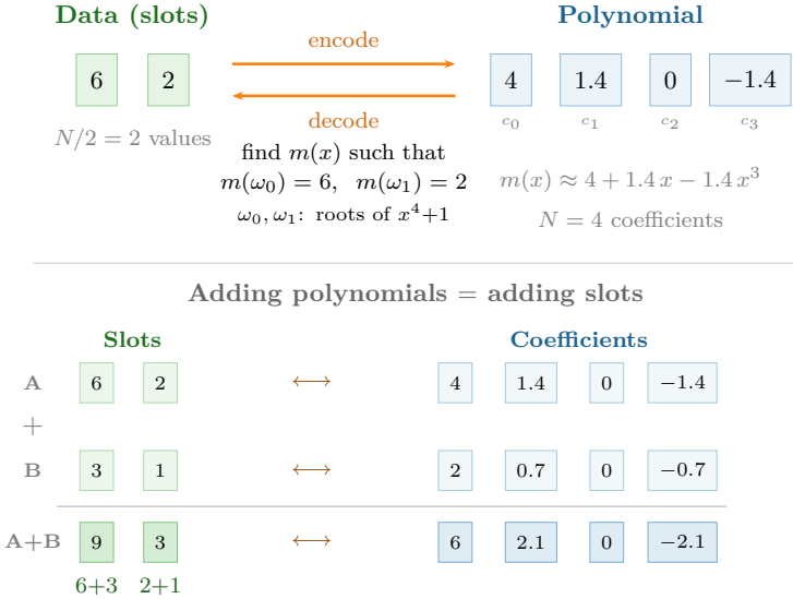
Figure 4.11: Slot-based encoding ( N = 4 ). Above: two data points [6, 2] are encoded as a polynomial with 4 coefficients by finding m(x) such that m(\omega_0) = 6 and m(\omega_1) = 2 . Below: adding two polynomials coefficient by coefficient is equivalent to adding the slots element by element — the basis of SIMD parallelism.
