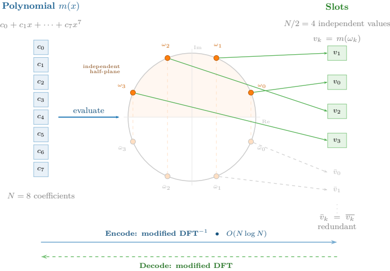
Figure 4.10: Canonical embedding. The polynomial m(x) 's coefficients are not the data: the slots are the evaluations of m(x) at the N complex roots of x^N + 1 . Conjugate roots produce redundant values, leaving N/2 independent slots. Encoding and decoding are equivalent to a modified DFT (inverse and direct, respectively).
