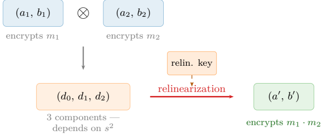
Figure 4.5: Multiplication between ciphertexts. The product generates a triplet (d_0, d_1, d_2) that depends on s^2 . Relinearization, using a public key that encrypts s^2 , reduces it to a standard pair (a', b') decryptable with s .
