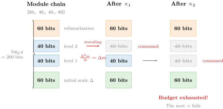
Figure 4.7: Modulus chain and level consumption. Each multiplication consumes one 40-bit link via rescaling. When the intermediate links run out, the next multiplication fails.
