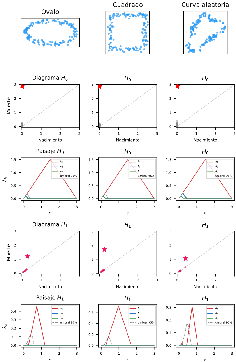
Figure 22.4: Topological invariance: an oval, a square, and a random curve — three different geometries with the same topology. In all cases, H_0 detects one component and H_1 detects a persistent cycle (star). The geometric shape changes; the topological shape does not.
