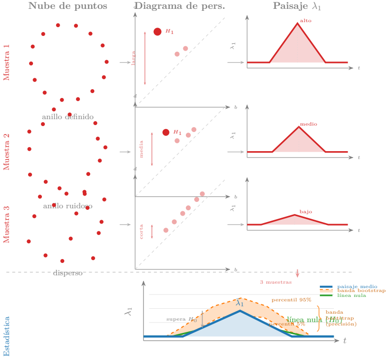
Figure 22.22: Three samples from the same process (rows 1–3) produce persistence diagrams with bars of different lengths and landscapes with peaks of different heights. The bottom row overlays the three individual landscapes (red) to obtain the mean landscape (blue), the bootstrap band 5%–95% (orange, variability band from resamples of the original dataset), and the null line (green, 95th percentile of landscapes from permuted data). The blue peak exceeds the null line — statistically significant signal — and stays within the bootstrap band — reproducible signal.
