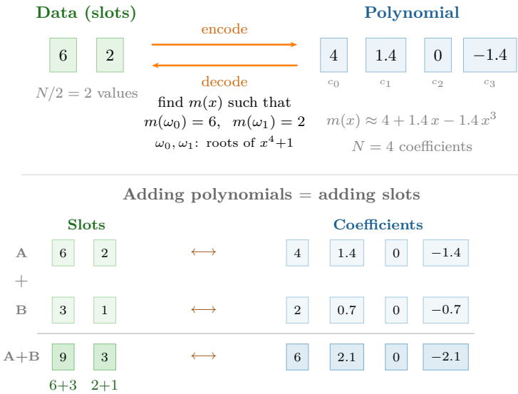
Figure 3.11: Slot-based encoding ( N = 4 ). Above: two data points [6, 2] are encoded as a polynomial with 4 coefficients by finding m(x) such that m(\omega_0) = 6 and m(\omega_1) = 2 . Below: adding two polynomials coefficient by coefficient is equivalent to adding the slots element by element — the basis of SIMD parallelism.
