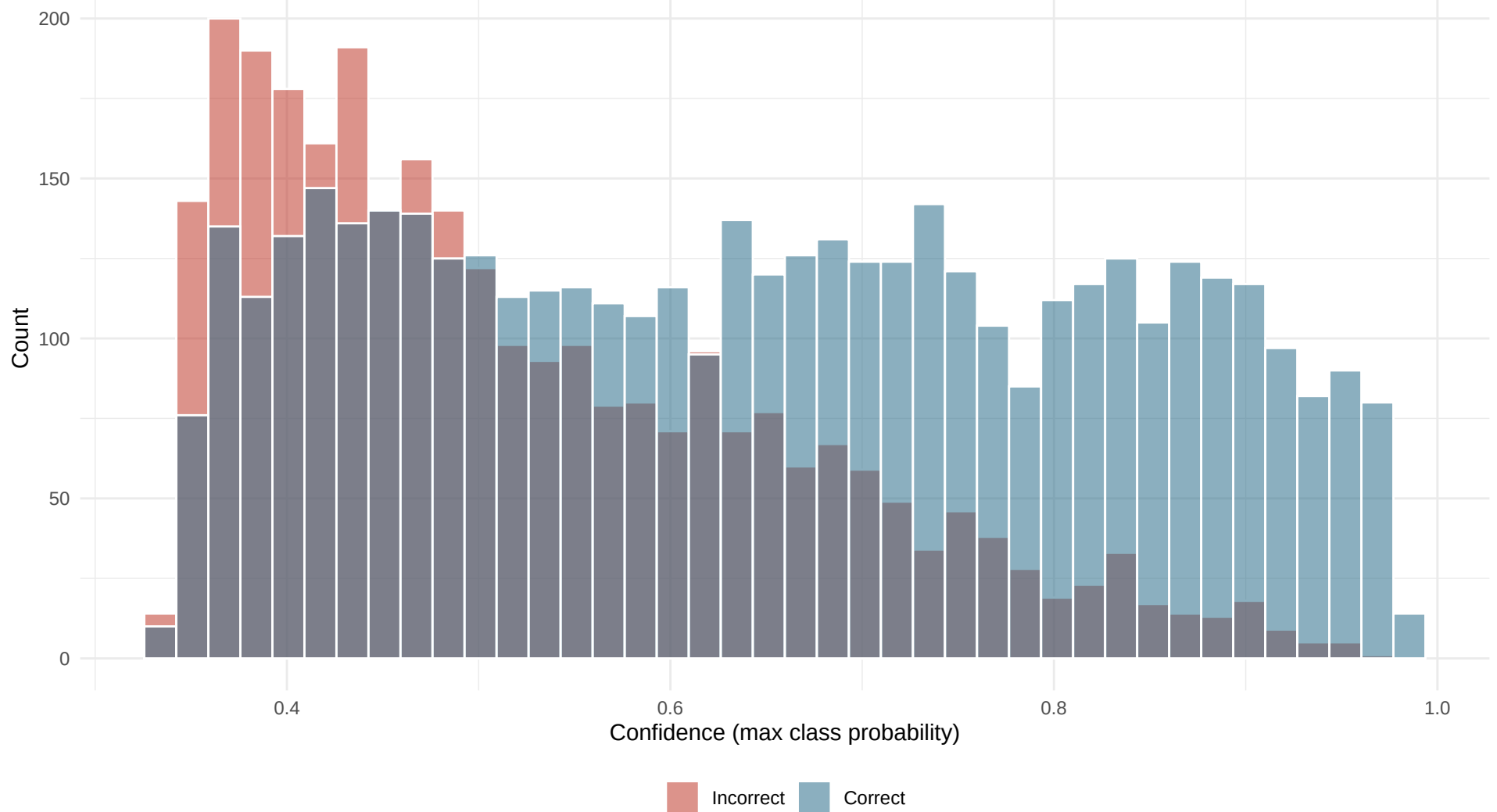
Prediction confidence distribution (best validation model, test split)
