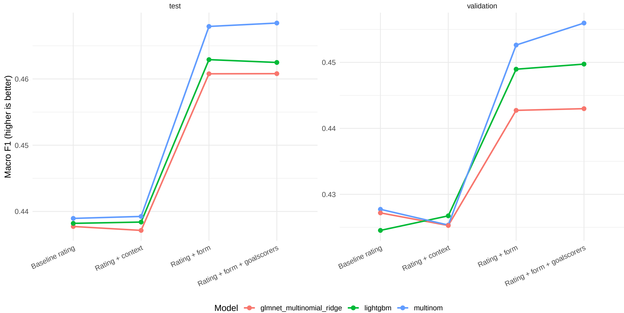
Incremental macro F1 by feature tier
