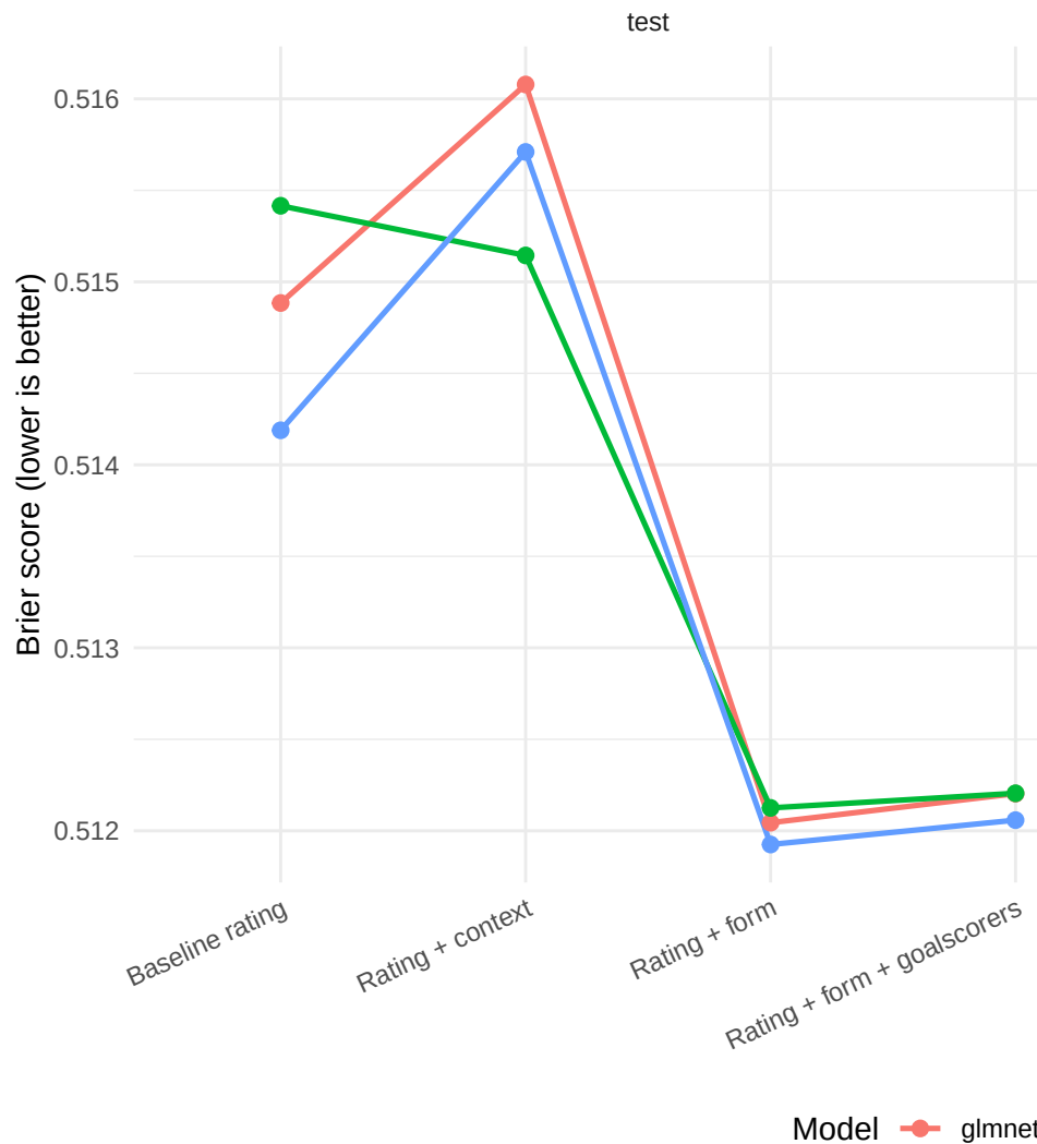
Incremental Brier score by feature tier
