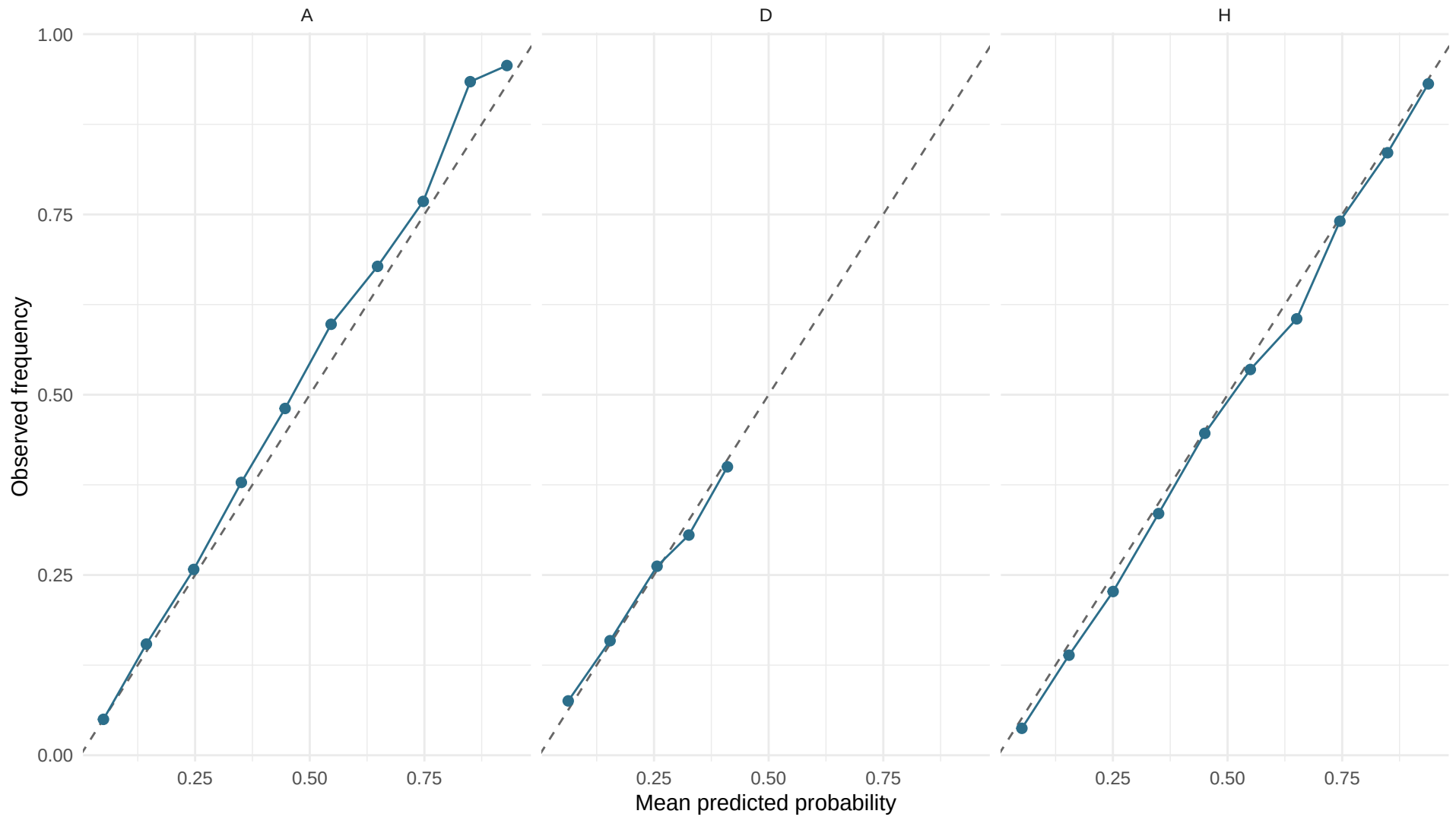
Calibration bins for best validation model (test split)
