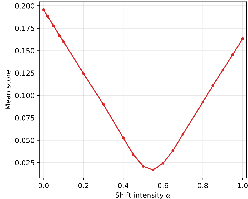
Embedding CIFAR-10-C
