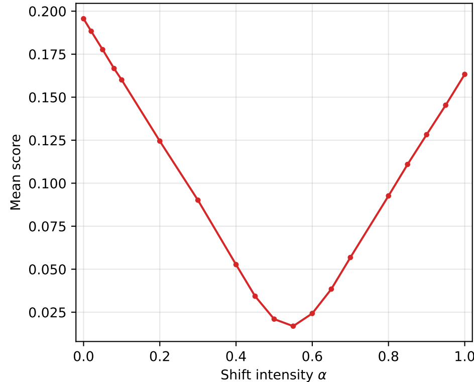
Embedding CIFAR-10
