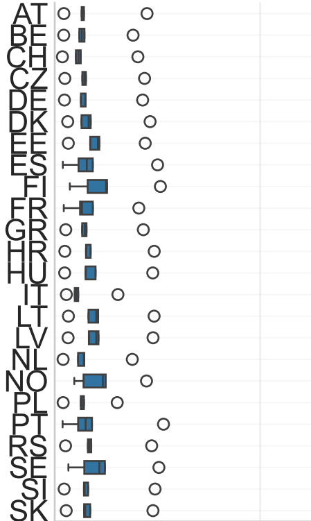
Hindcast-dynamic
