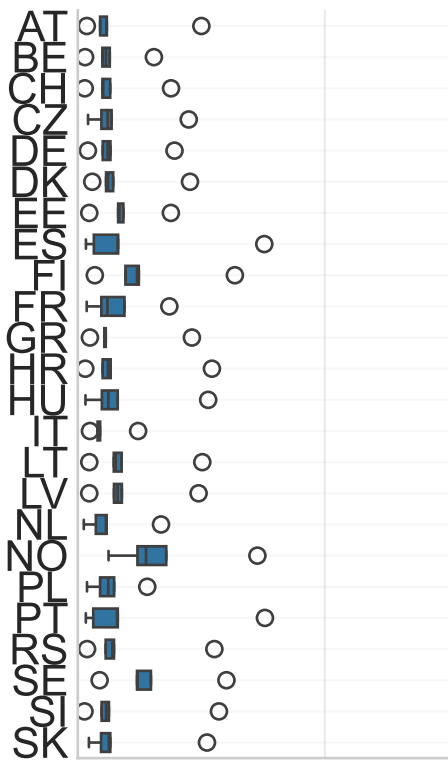
rmse
