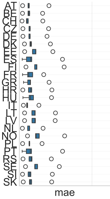
Hindcast-dynamic-rolling horizon
