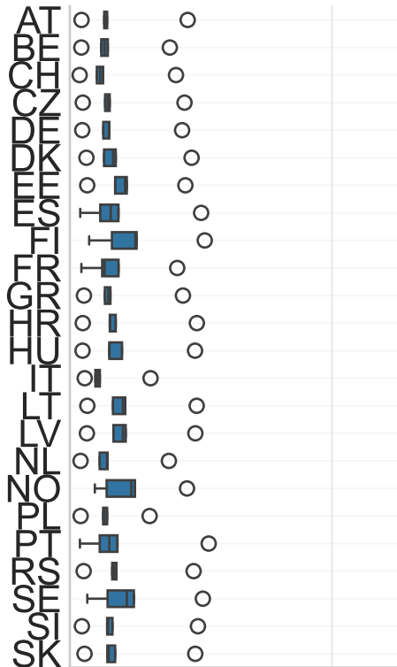
Hindcast-dynamic
