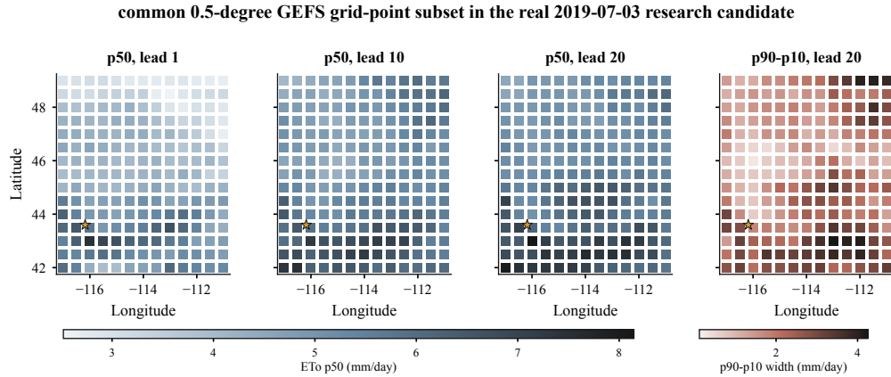
Figure 4. Reference- ET_0 fields for the real 2019-07-03 candidate on the common 0.5-degree GEFS grid-point subset. The first three panels show p50 at leads 1, 10, and 20. The last panel shows p90 minus p10 at lead 20. Each panel contains n = 195 grid points. No interpolation, field geometry, or area-weighted Idaho estimate is inferred.
