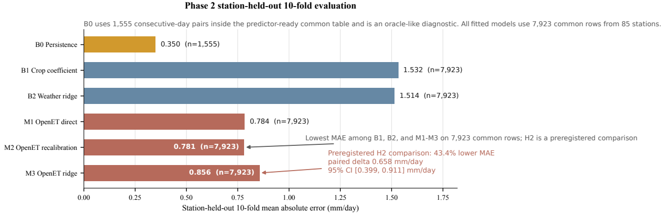
Figure 2. Station-held-out actual-ET MAE. B2 and M3 form the preregistered H2 comparison. Their common sample contains n = 7,923 rows from 85 stations. M2 has the lowest MAE among B1, B2, and M1 through M3 on 7,923 common fitted-model rows. It does not inherit the M3 interval. B0 uses n = 1,555 consecutive-day pairs inside the predictor-ready common table. It is excluded from H2.
