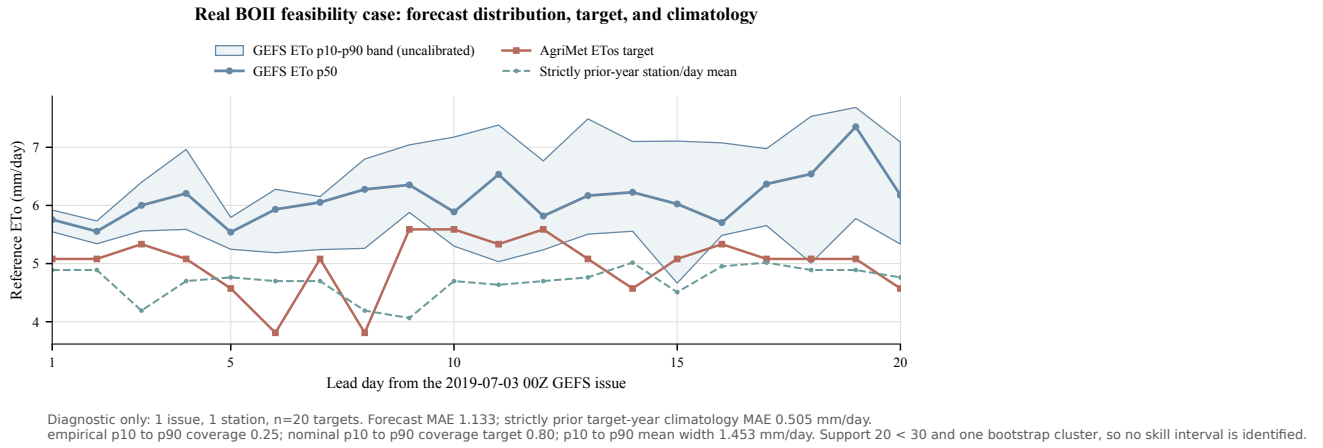
Figure 3. One real BOII feasibility case. The GEFS member distribution gives p10, p50, and p90 reference ET_0 for leads 1 through 20. The independent target is AgriMet ET_0 s. The baseline uses the same station and target day of year with observations from strictly prior calendar years. The scope is one issue, one station, and n = 20 targets. It is diagnostic only.
