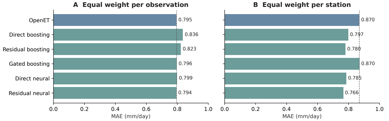
Figure 10. The weighting rule changes the joint-transfer conclusion on identical observations. The dashed line marks unchanged OpenET. Residual boosting worsens pooled MAE but improves the station-weighted point estimate. Table 5 supplies paired uncertainty intervals.
