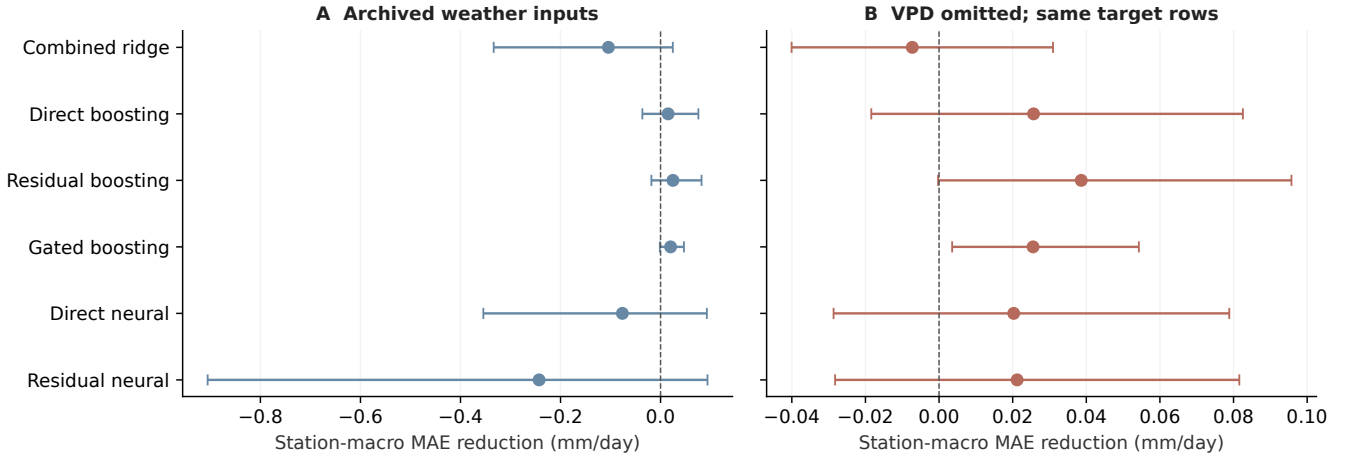
Figure 8. Paired 95% intervals for station-MAE reductions against unchanged OpenET. The primary proximity split evaluates identical target rows in both panels. Left: archived weather inputs. Right: refits without VPD. The horizontal scales differ to display the large original uncertainty and the smaller remaining effects.
