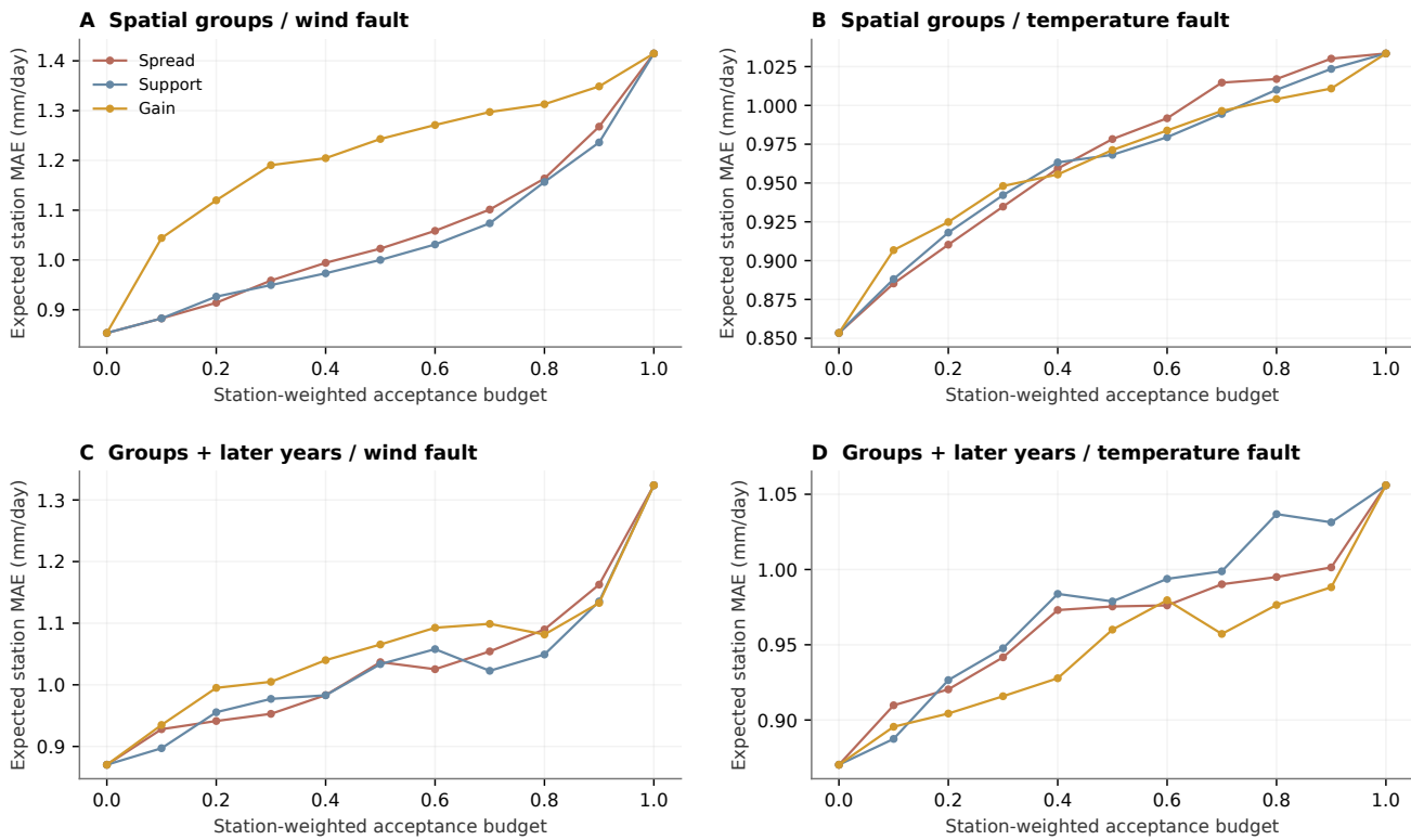
Figure 5. Expected station MAE at matched station-weighted acceptance budgets, with VPD omitted. The boundary decision is randomized to match each budget exactly. Every other rejected correction returns OpenET. These post hoc curves use label-free outer ranks; they do not establish deployable thresholds. The paired 50% comparisons appear in the text.
