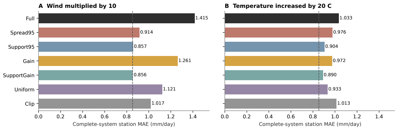
Figure 4. Paired input faults on 7,873 eligible proximity-test observations after VPD omission. The dashed line is unchanged OpenET. Each complete system includes its fallback predictions. Different acceptance rates contribute to these differences. Table 10 reports the other evaluation and the exact negative control.
