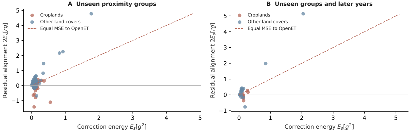
Figure 9. Exact squared-error diagnostics for original-input residual boosting. Both axes have units (\text{mm day}^{-1})^2 . Each point is one test station; color identifies croplands versus other land covers. A full correction improves station MSE only above the diagonal. Test moments are explanatory and never select the reported gate.
