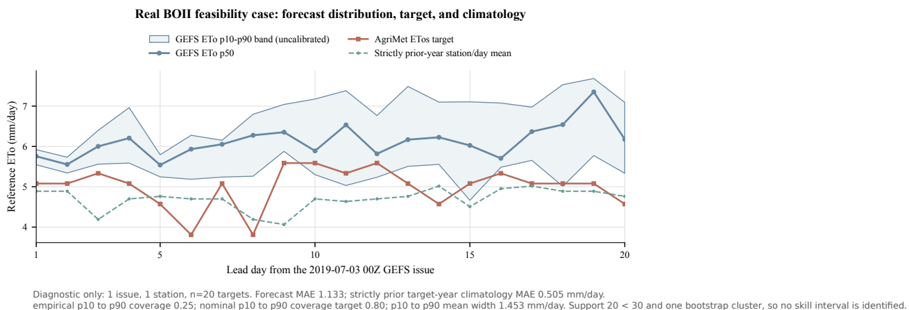
Figure 11. One real BOII feasibility case. The GEFS member distribution gives p10, p50, and p90 reference ET_o for leads 1 through 20. The independent target is AgriMet ETos. The baseline uses the same station and target day of year with observations from strictly prior calendar years. The scope is one issue, one station, and n = 20 targets. It is diagnostic only.
