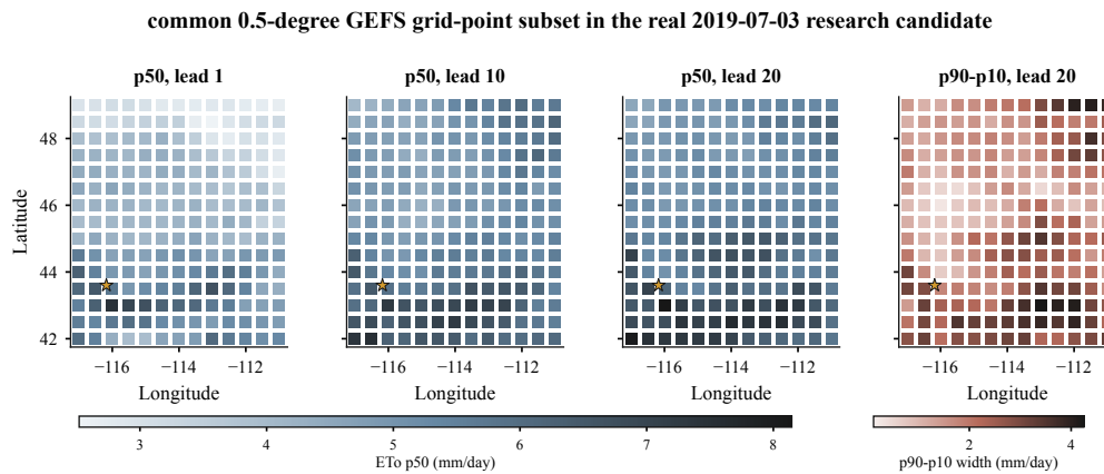
Figure 12. Reference-ET 0 fields for the real 2019-07-03 candidate on the common 0.5-degree GEFS grid-point subset. The first three panels show p50 at leads 1, 10, and 20. The last panel shows p90 minus p10 at lead 20. Each panel contains n = 195 grid points. No interpolation, field geometry, or area-weighted Idaho estimate is inferred.
