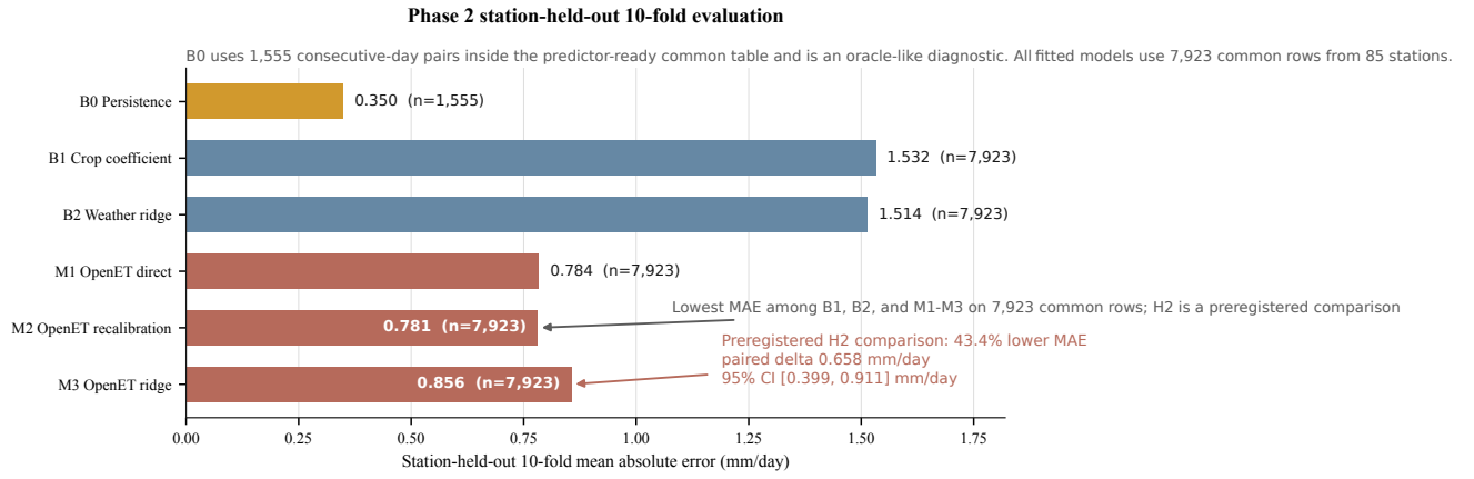
Figure 6. The original station-held-out model visual, retained unchanged. H2 (the preregistered OpenET comparison) concerns B2 weather ridge and M3 combined ridge. Its matched sample has 7,923 rows. The previous-label persistence diagnostic uses 1,555 pairs and is not a matched correction baseline.
