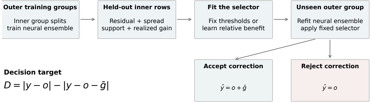
Figure 2. The selective residual experiment. Inner spatial cross-fitting supplies the selection data. Outer targets are used only for evaluation. Every rejected correction returns unchanged OpenET.
