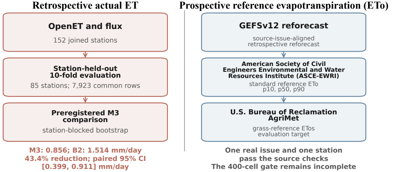
Figure 1. The original MLET evidence architecture, retained unchanged. The left branch supplies 7,923 station-days from 85 stations for retrospective actual-ET evaluation. The right branch contains a separate reference-ET 0 protocol and one diagnostic with 20 targets. The new selective neural experiments concern the left branch.
