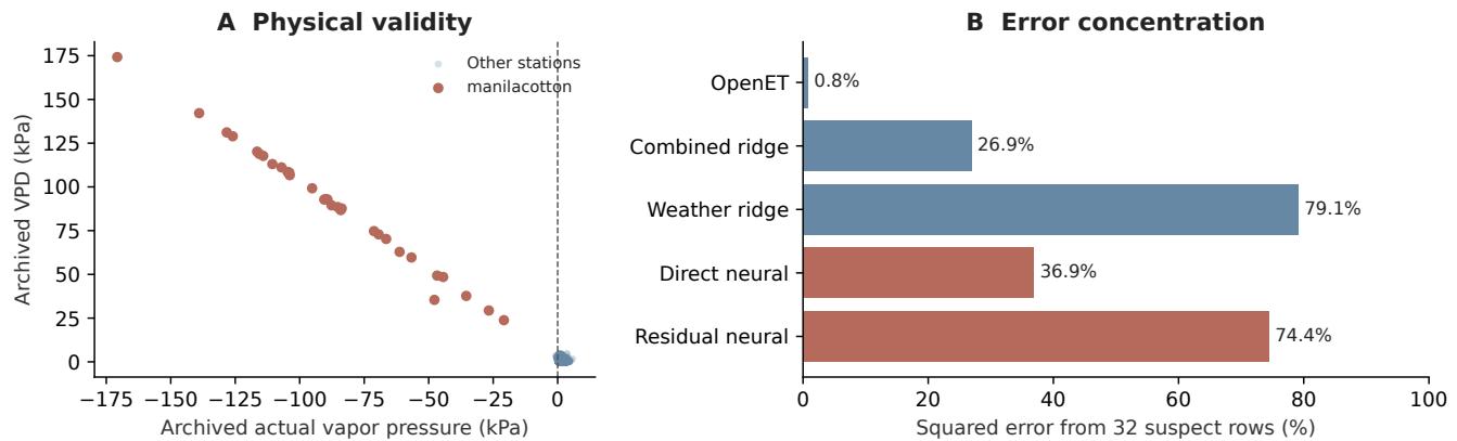
Figure 7. Input validity and error concentration in the primary split. Left: archived actual vapor pressure and VPD on selected dates. Right: squared-error shares from 32 observations at the suspect station. The source values support a physical-inconsistency diagnosis, not an identified conversion factor.
