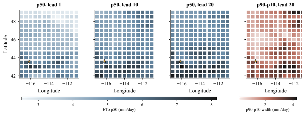
common 0.5-degree GEFS grid-point subset in the real 2019-07-03 research candidate
