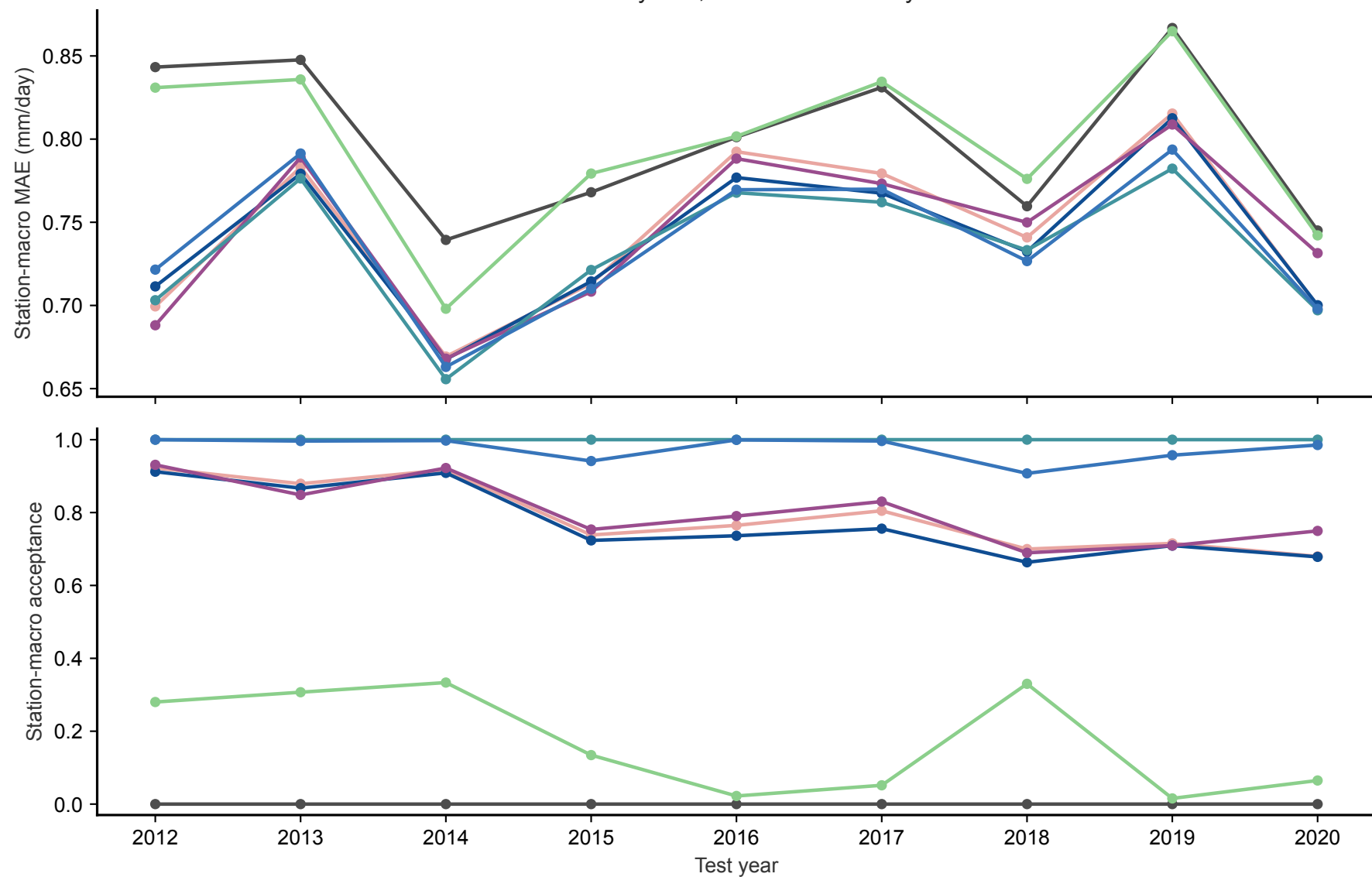
Annual test years, trained on earlier years
