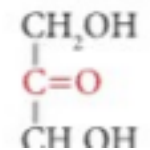
\text{CH}_2\text{OH} diidrossiacetone
