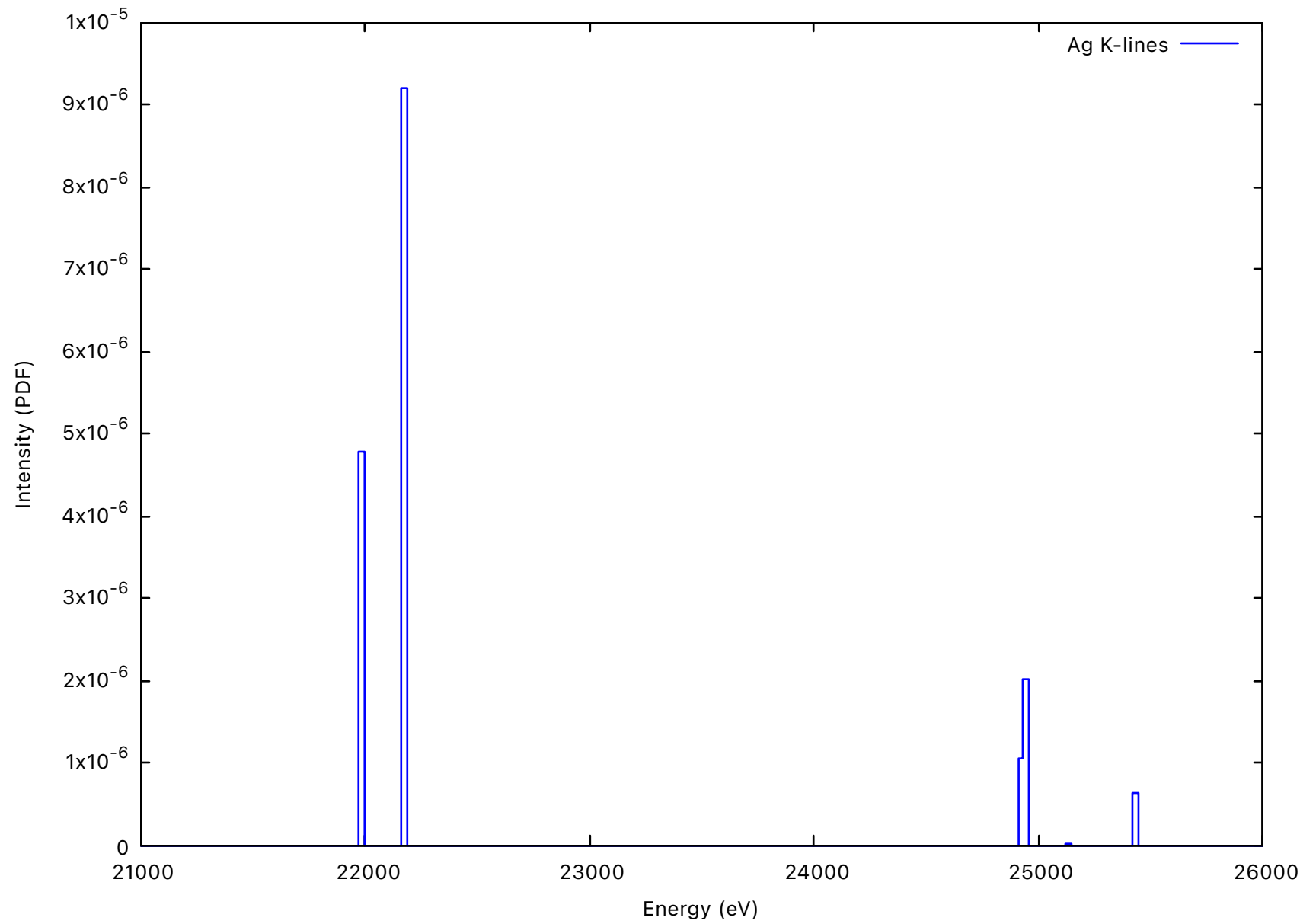
Silver PIXE Spectrum (10 MeV Protons)
