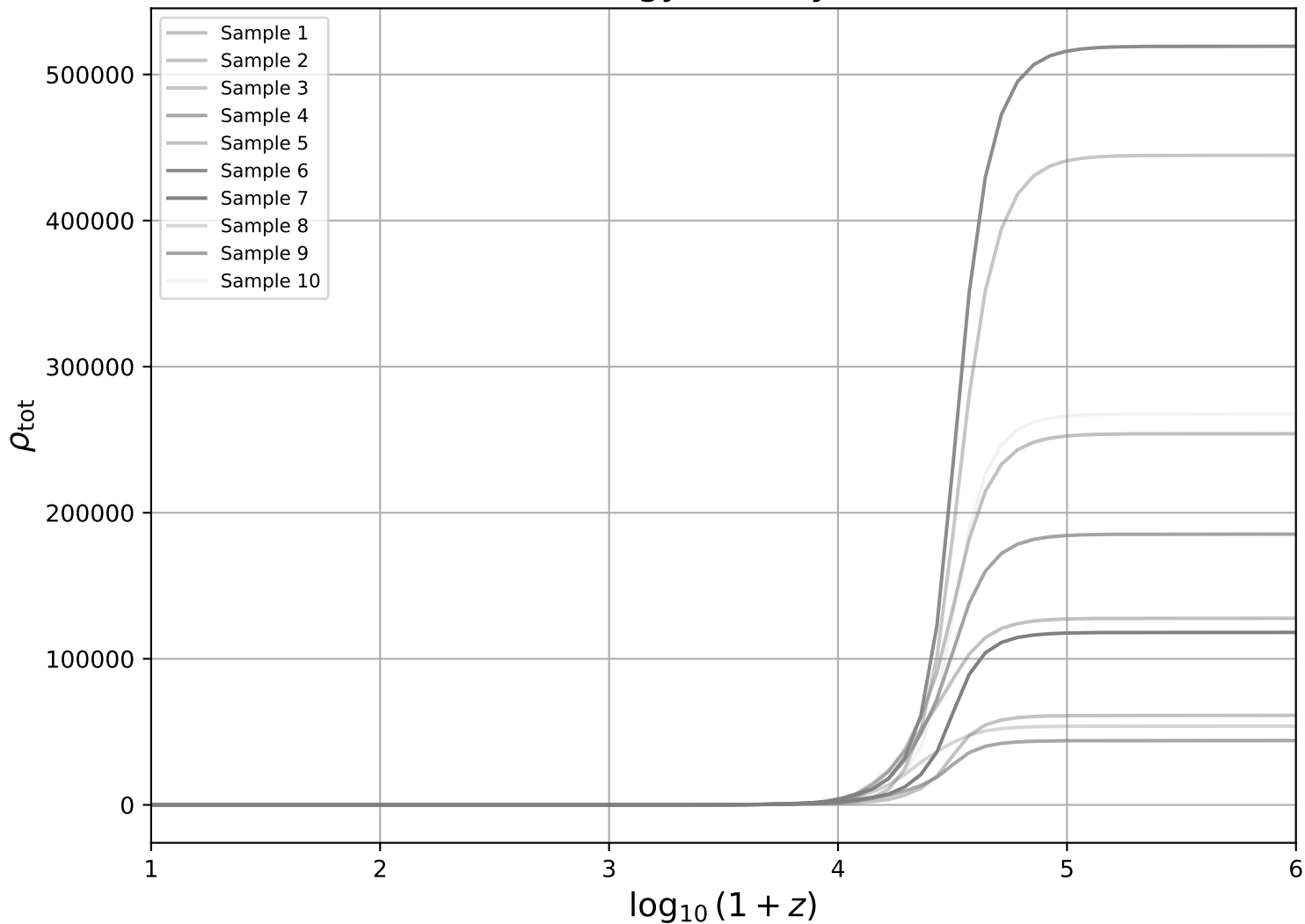
Total EDE energy density over redshift
