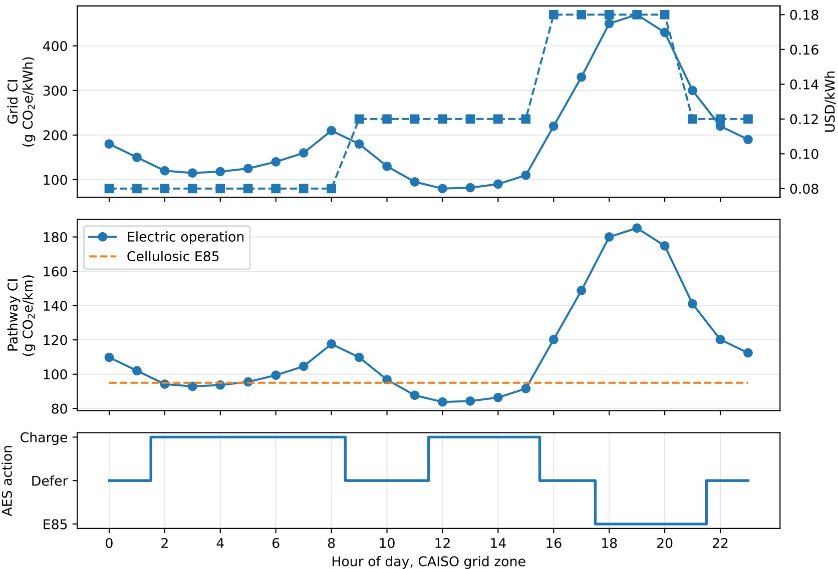
Time-resolved grid carbon intensity and AES dispatch decisions
