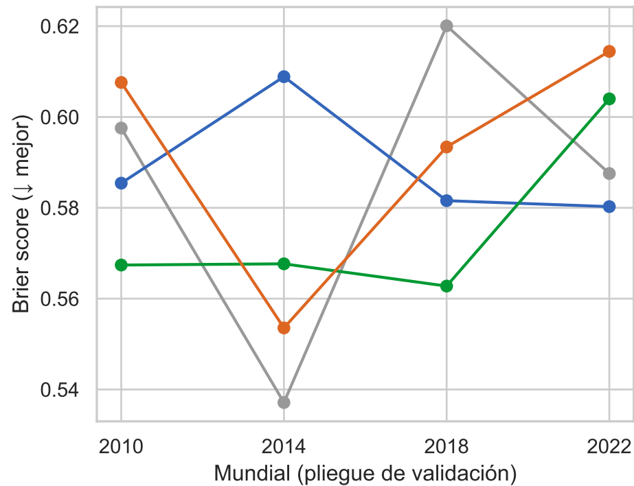
Brier score
