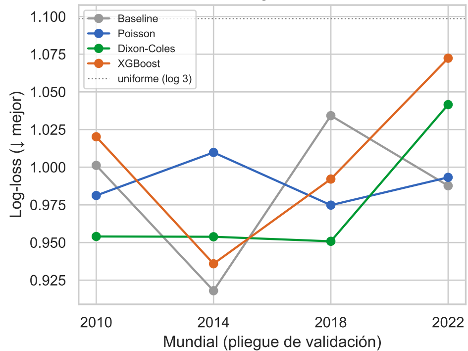
Log-loss
