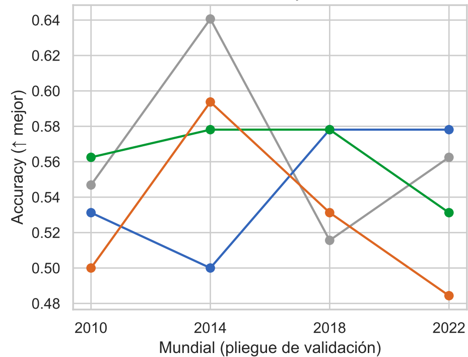
Accuracy
