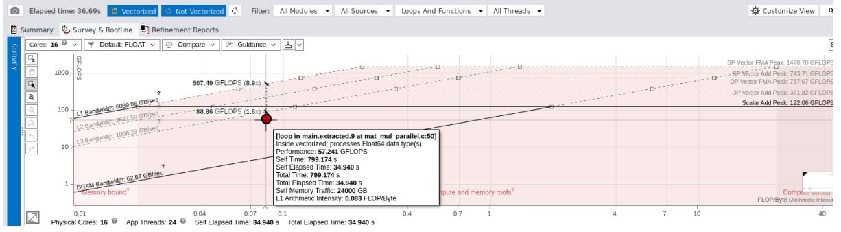
Figure 8: Roofline Model of the first parallel execution ( N = 10000 ).
