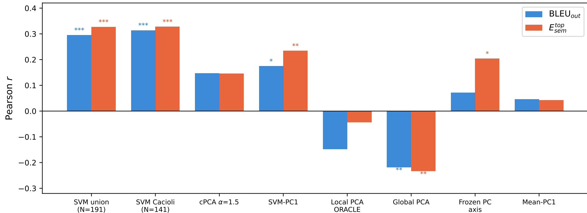
Cacioli Ablation: Drift Axis Methods ( N = 141 , ONLINE)
