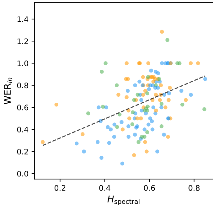
Cacioli Corpus ( N = 141 ): H_{\text{spectral}} vs. Quality Metrics ( \text{WER}_{in} and E_{sem}^{top} )
