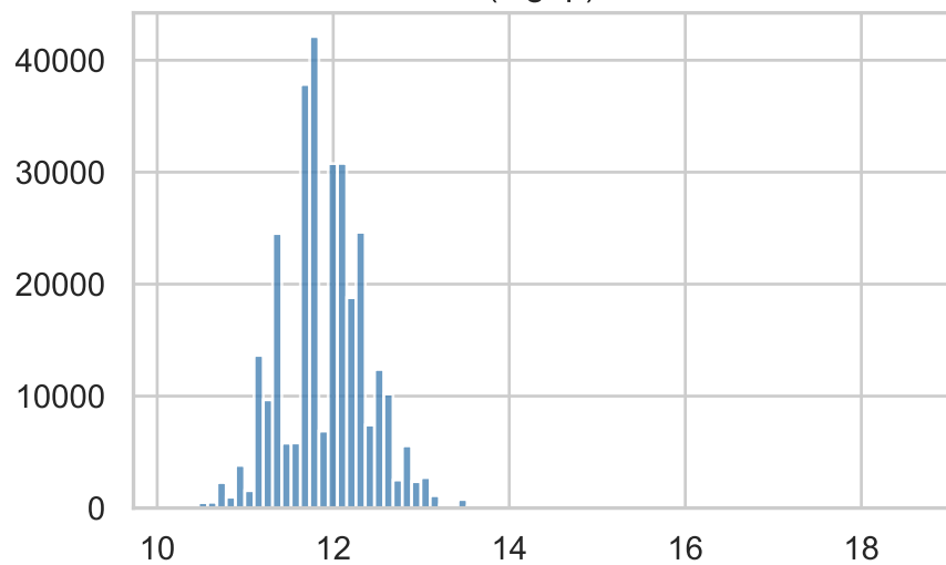
AMT_INCOME_TOTAL (log1p)
