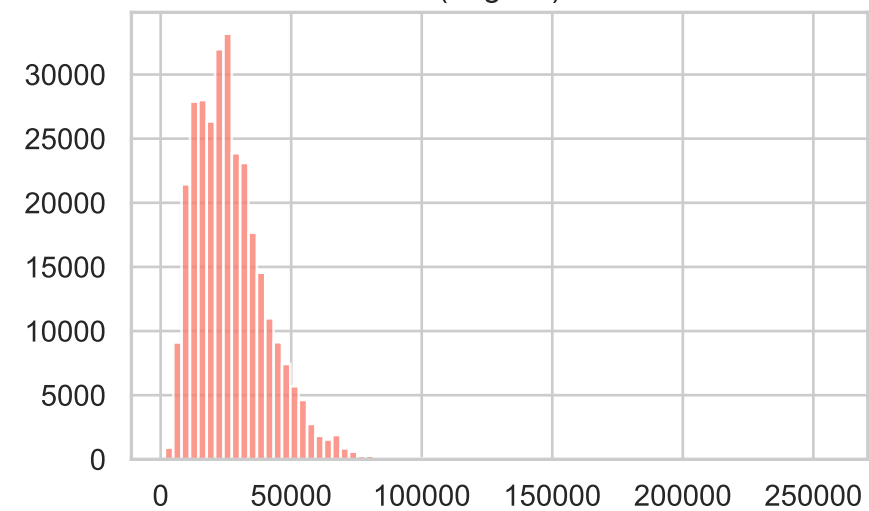
AMT_ANNUITY (original)
