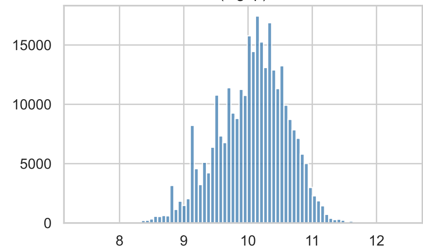
AMT_ANNUITY (log1p)
