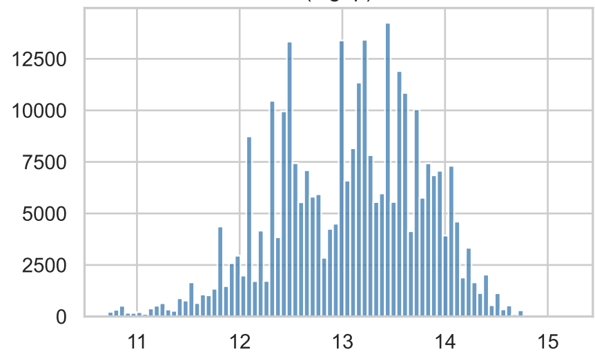
AMT_CREDIT (log1p)
