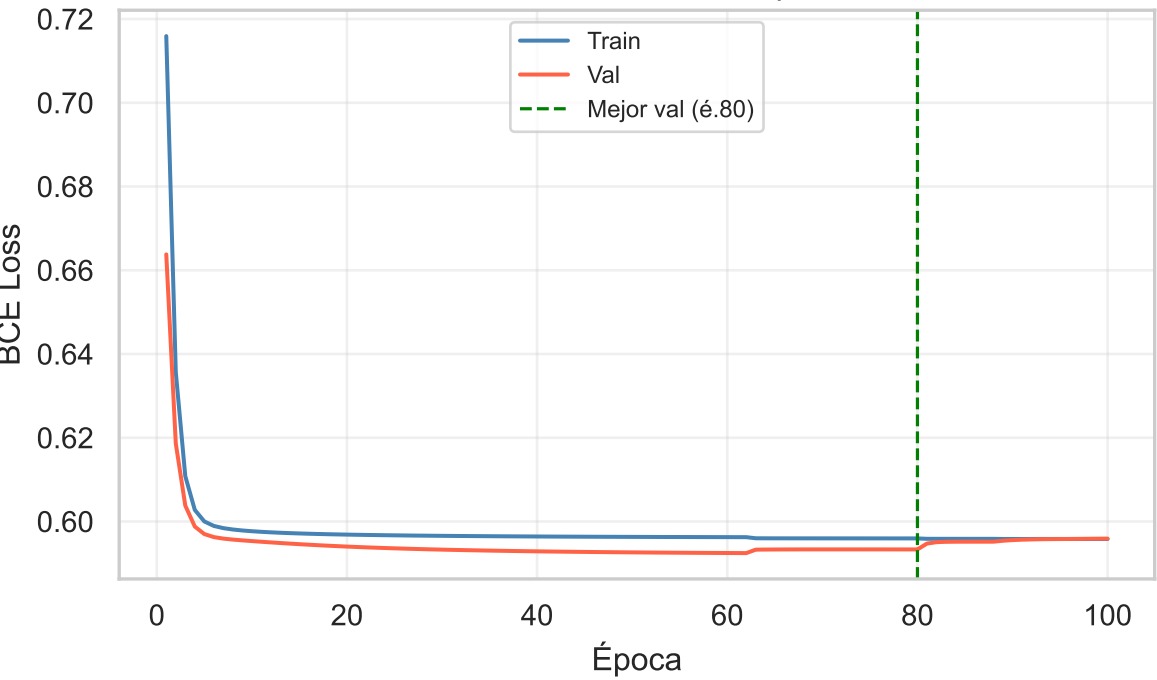
BCE Loss — Curva completa
