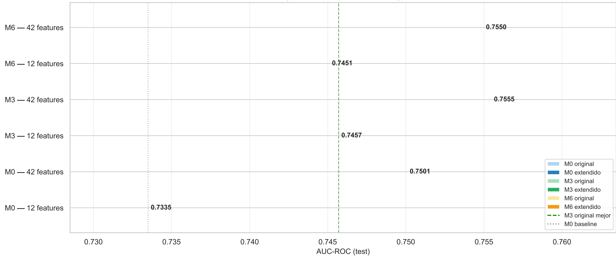
12 features originales vs 42 features extendidas (colores oscuros = extendido)
