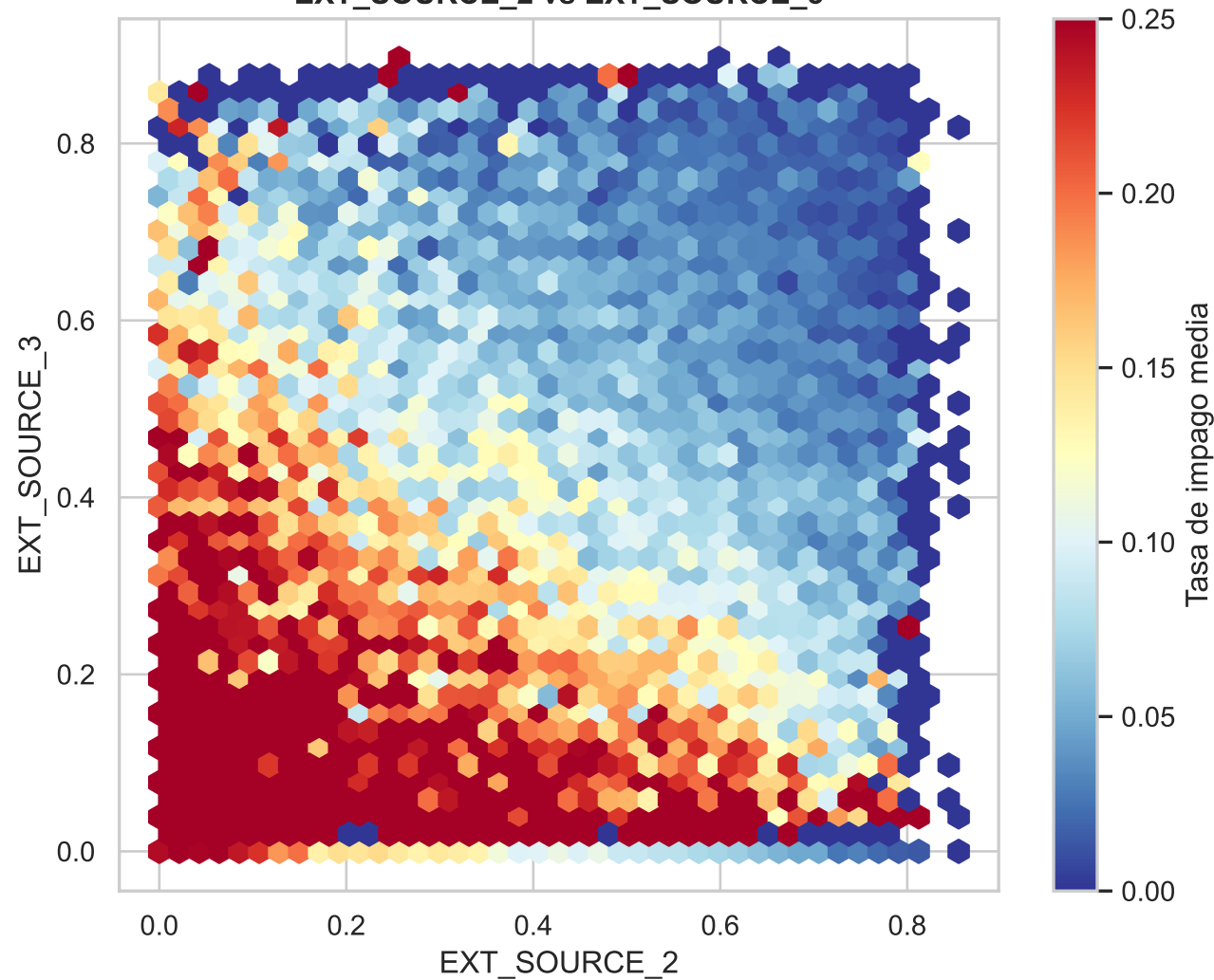
Hexbin: tasa de impago EXT_SOURCE_2 vs EXT_SOURCE_3
