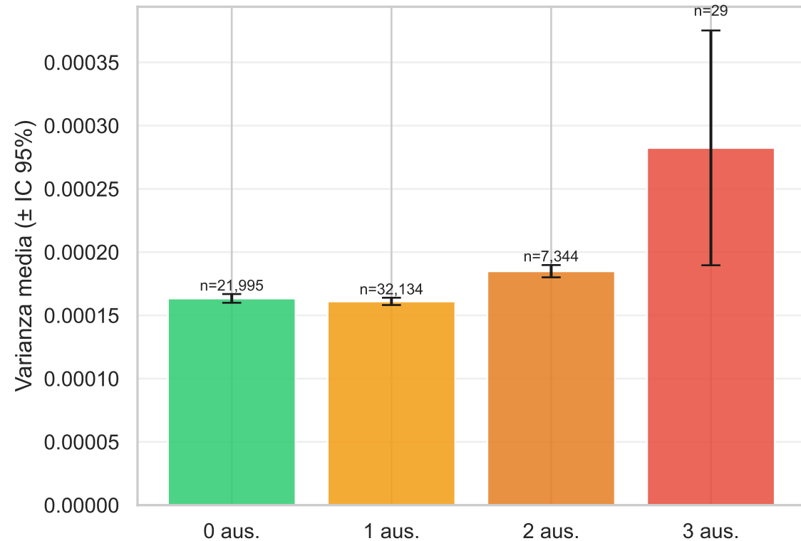
FAIR \lambda=0.5
