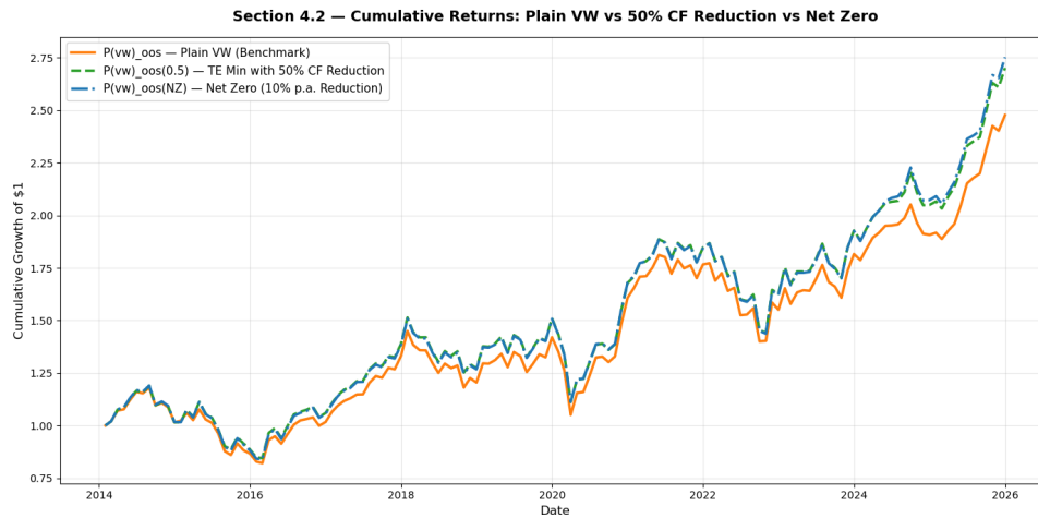
Figure 11: Cumulative Returns Comparison: VW Benchmark, 50% CF Reduction, and Net Zero Strategy.
