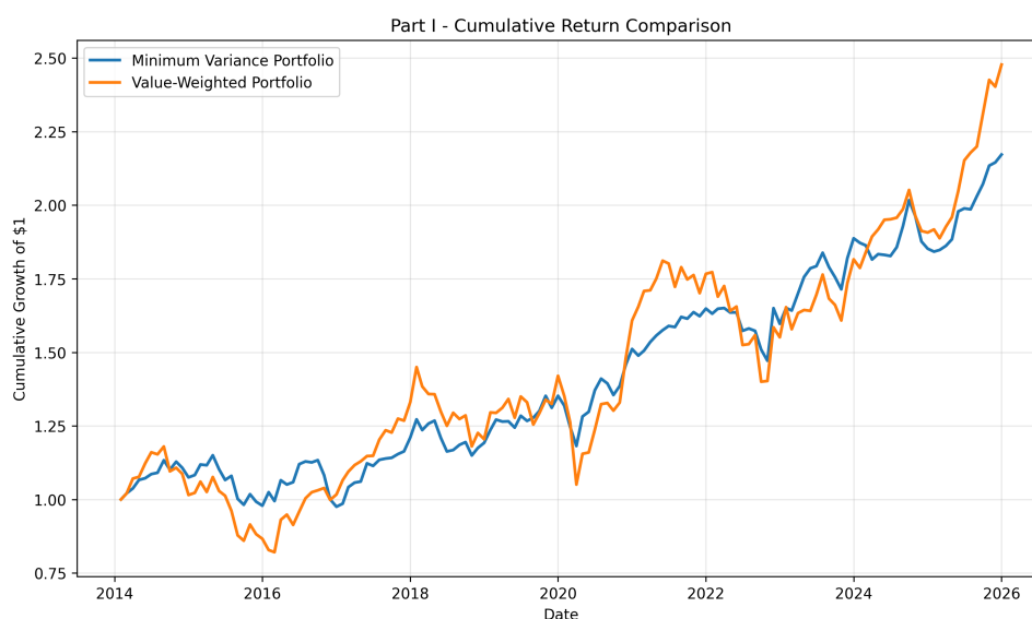
Figure 1: Cumulative return comparison
