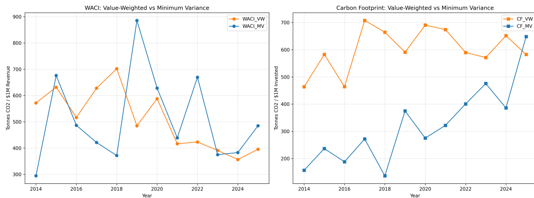
Figure 4: Annual WACI and carbon footprint of the two baseline portfolios, P_{\text{oos}}^{(\text{mv})} and P^{(\text{vw})} , over 2014–2025.
