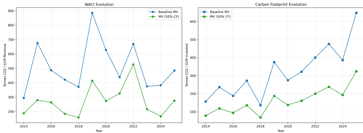
Figure 6: WACI and carbon footprint evolution of P_{\text{oos}}^{(\text{mv})} and P_{\text{oos}}^{(\text{mv})}(0.5) .
