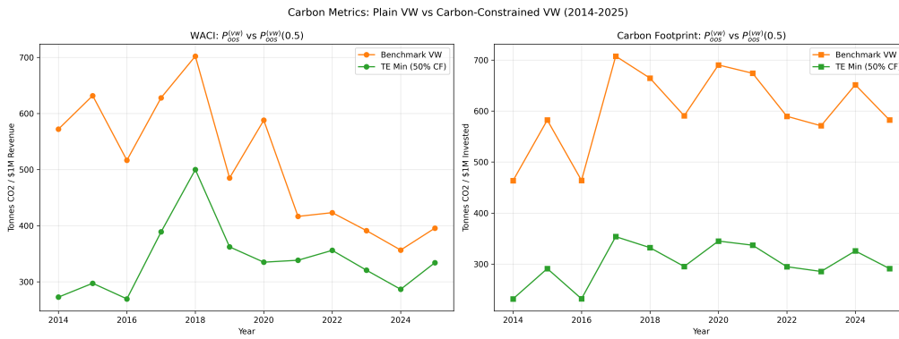
Figure 8: WACI and carbon footprint evolution of P^{(vw)} and P_{00s}^{(vw)}(0.5) .
