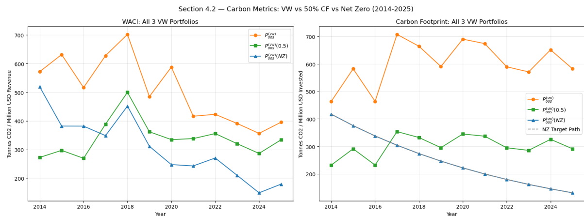
Figure 10: Environmental Trajectories: WACI for the three portfolios over time (left) and Carbon Footprint over time (right).
