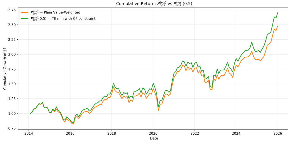
Figure 7: Cumulative returns of P^{(vw)} and P_{00s}^{(vw)}(0.5) .
