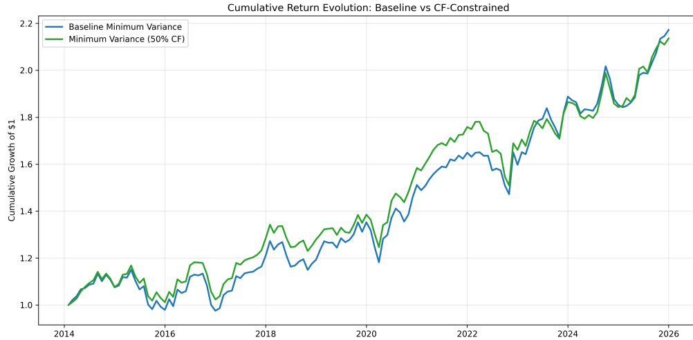
Figure 5: Cumulative returns of P_{\text{oos}}^{(\text{mv})} and P_{\text{oos}}^{(\text{mv})}(0.5) .
