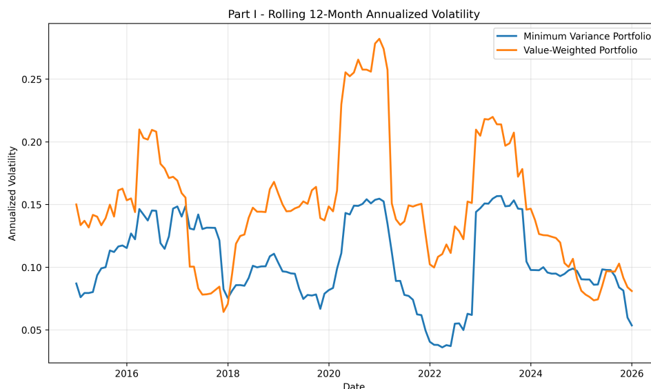
Figure 2: Rolling 12-month annualized volatility
