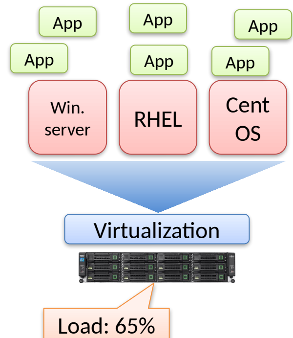
Virtualization
