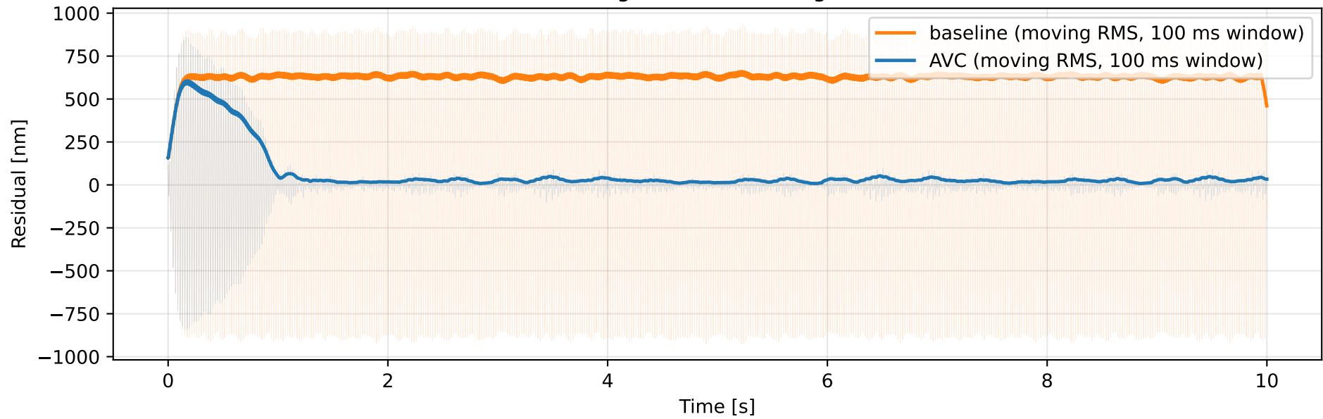
Overall residual (RMS across all 40 modes) vs. time (faint: raw signal, bold: moving RMS trend)
