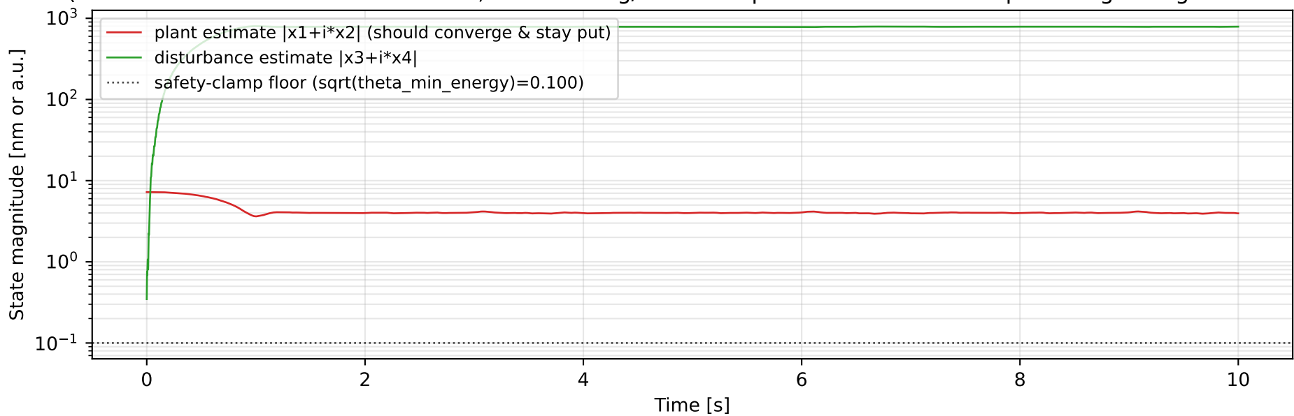
AVC internal state: is the online plant estimate ( x_1, x_2 ) stable?
