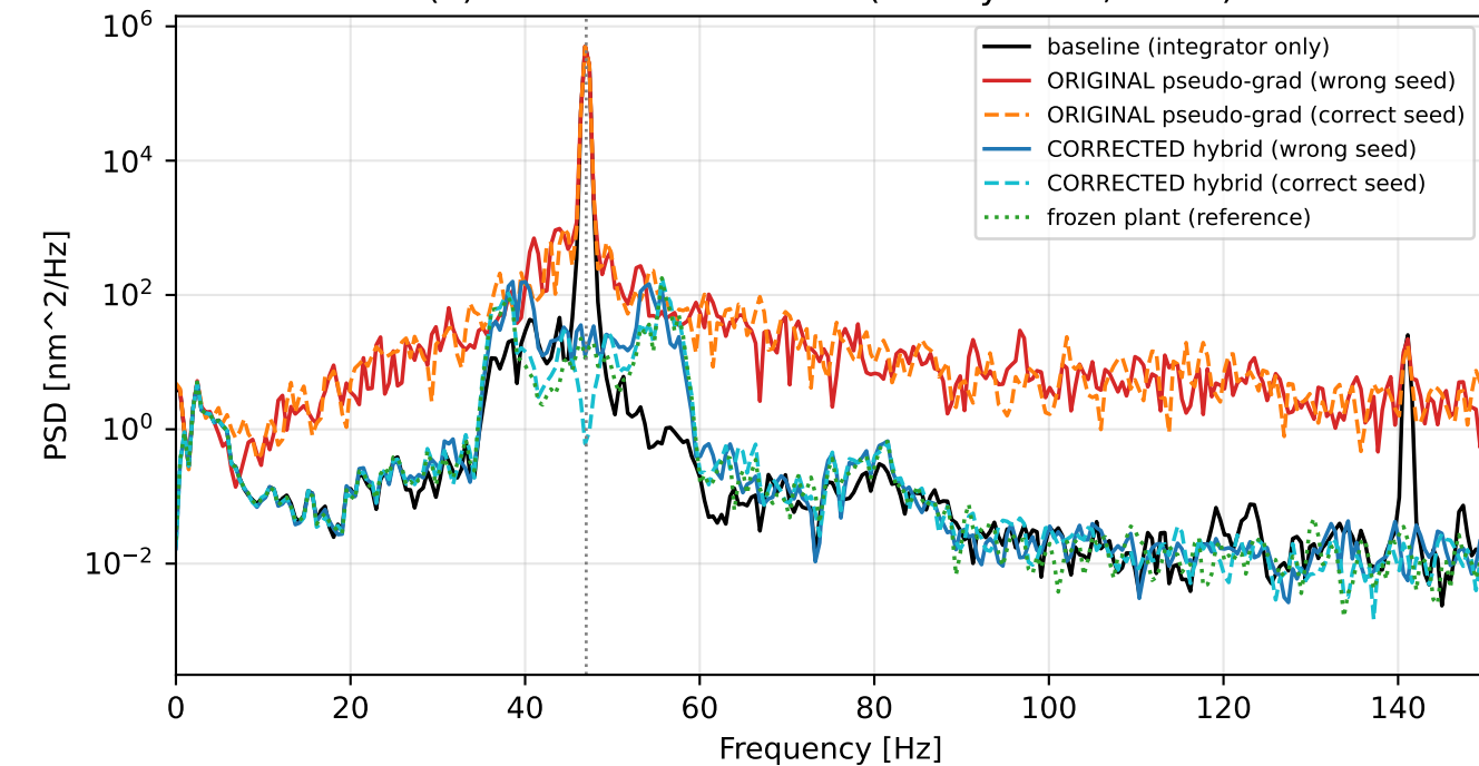
(e) Mode-0 residual PSD (steady state, t > 5 s)
