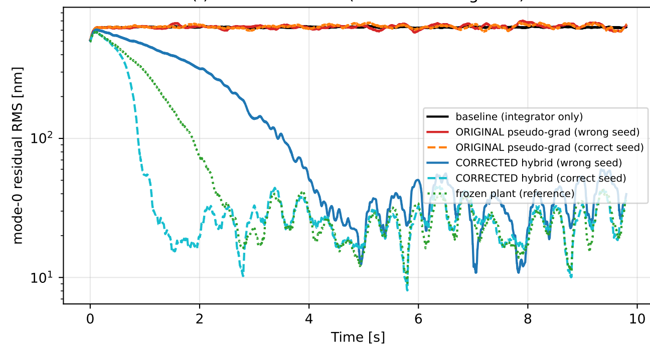
(f) Mode-0 residual (200 ms moving RMS)
