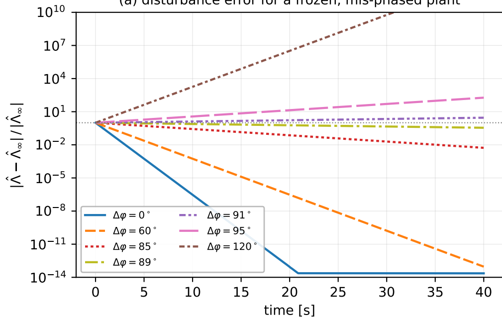
(a) disturbance error for a frozen, mis-phased plant
